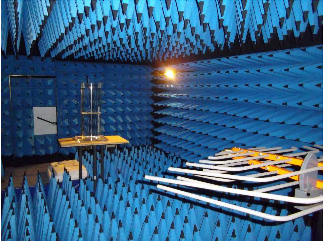
Radiated test set up photograph
