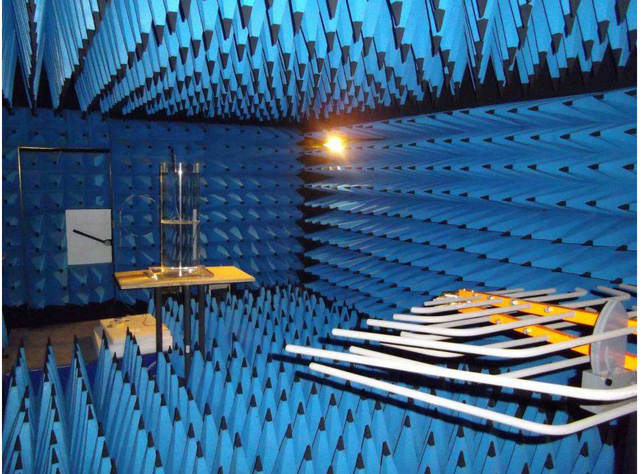
Radiated test set up photograph
