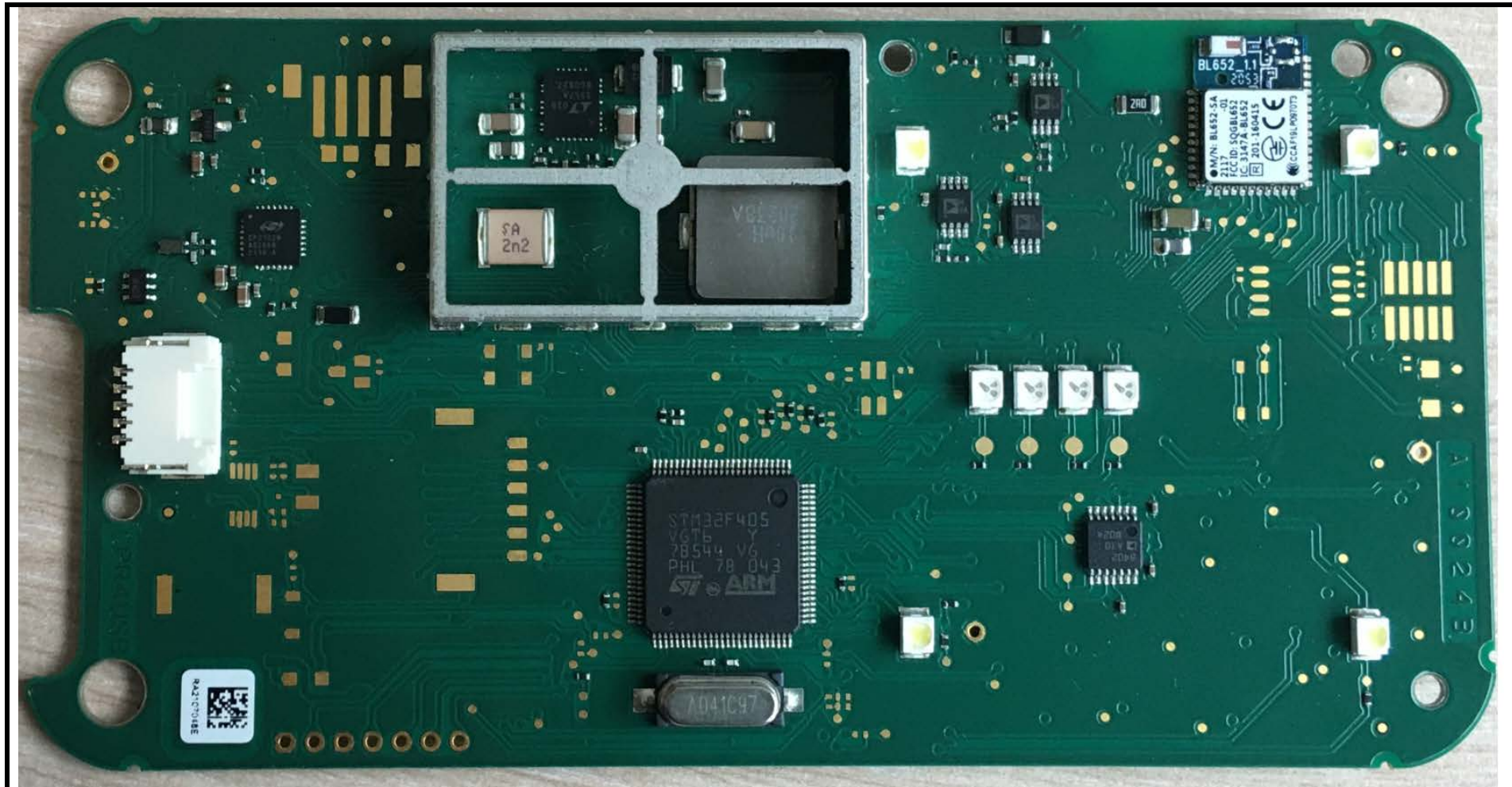
1 – PCB top view. BLE module top-right corner BL652
