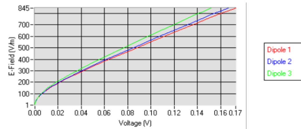
Calibration curves
