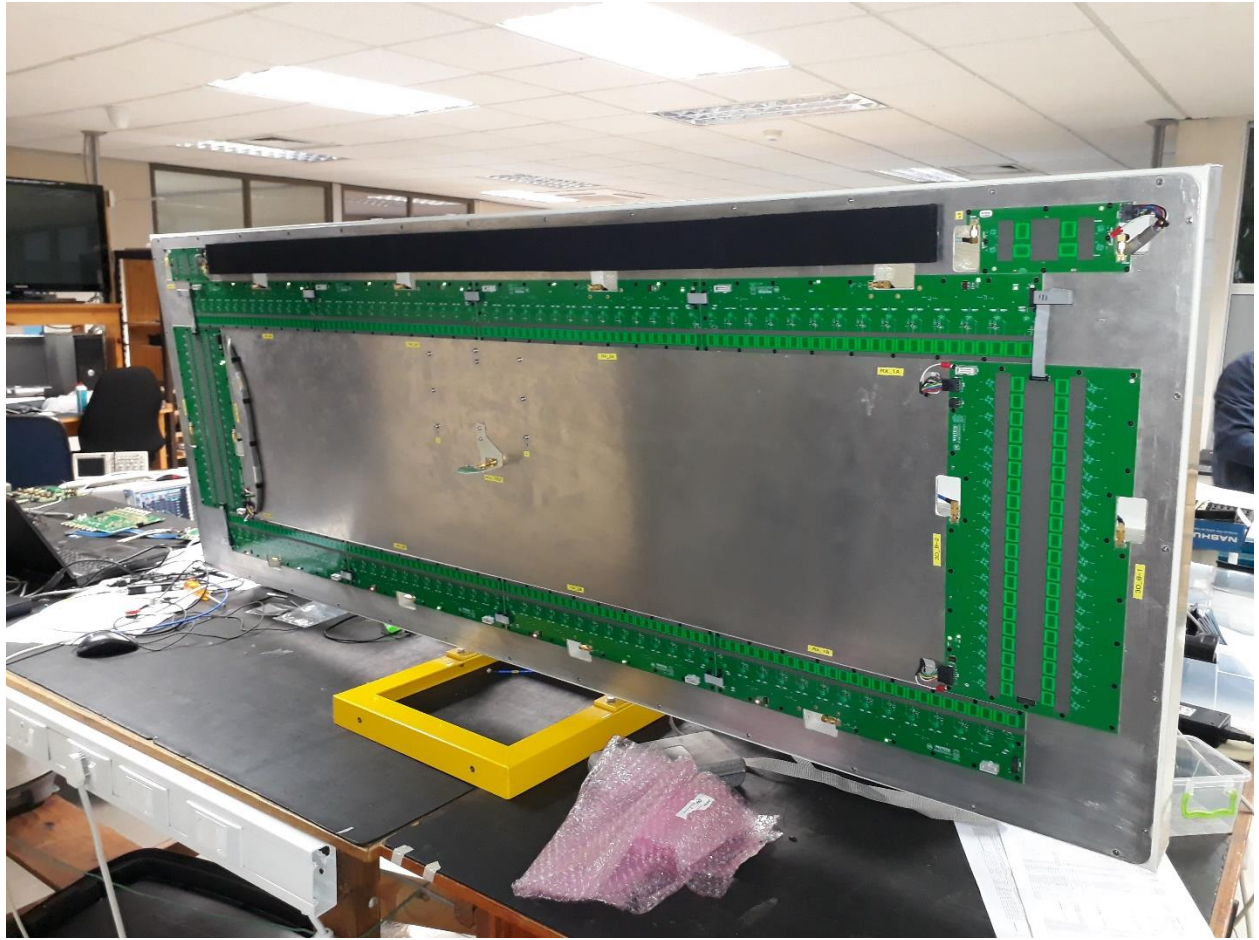
RFU Front View without Radome
