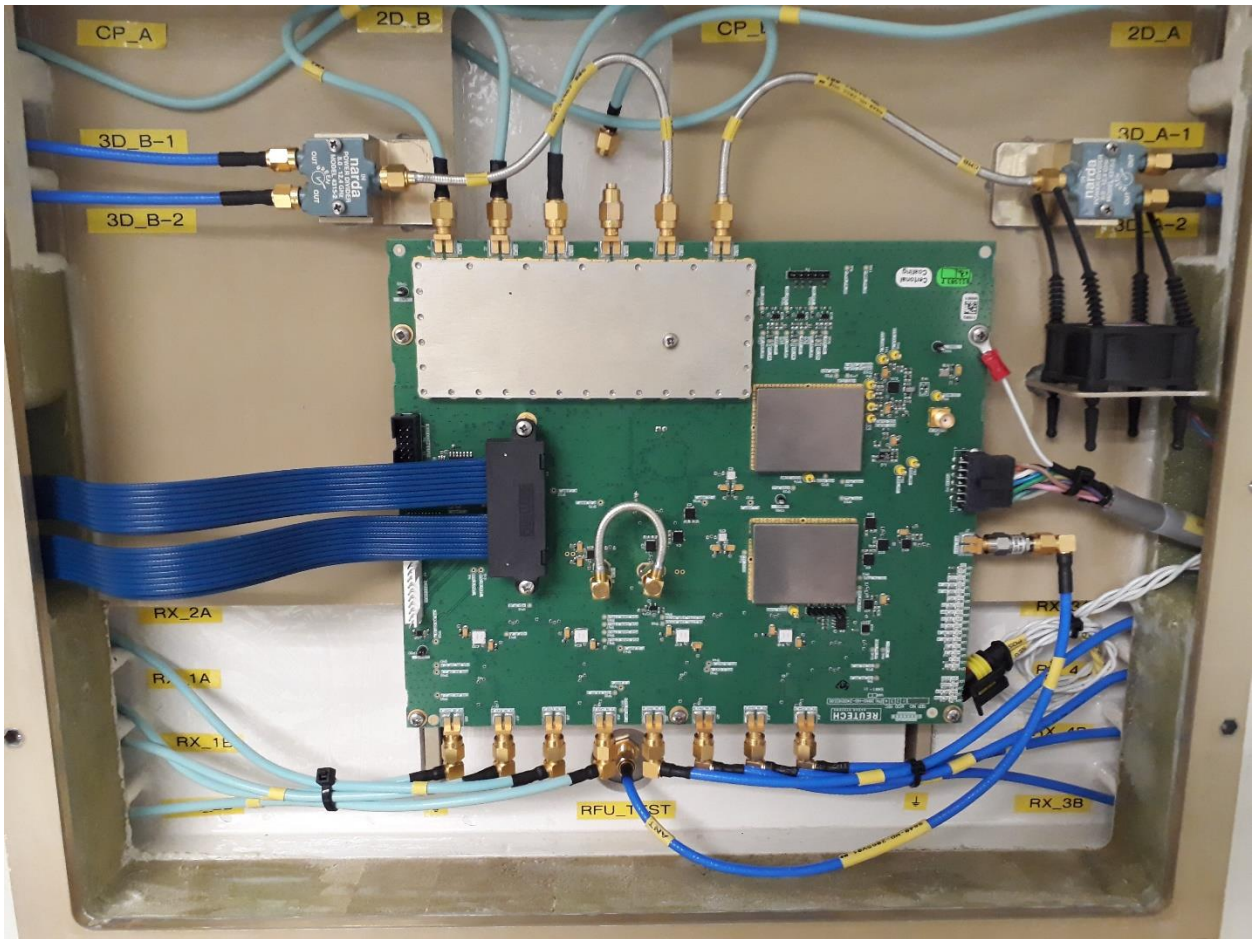
TRX Inside RFU
