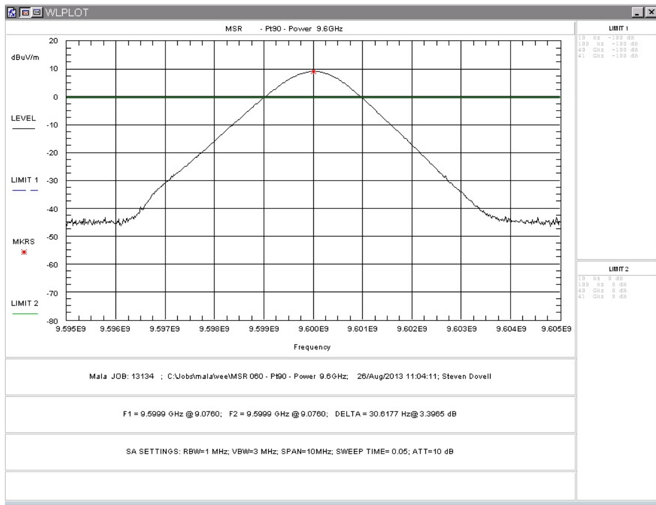
Figure 4-2. RF Peak Power, Mid Channel
