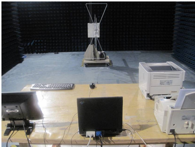
Test Setup Back View
