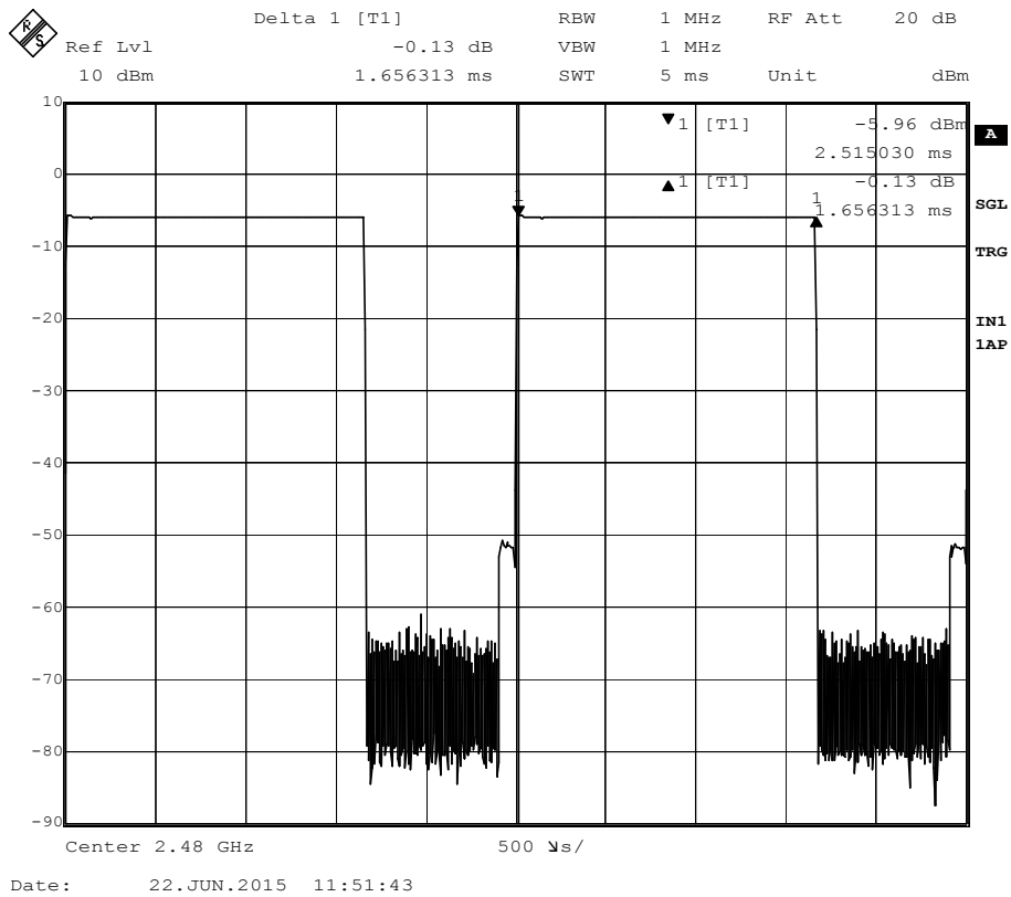
Fig. F [Pulse duration of Highest Channel] Pulse duration = 1.656ms
