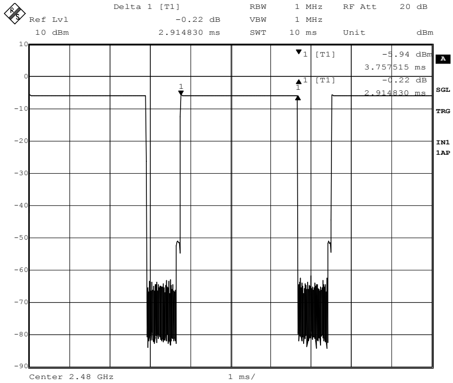
Fig. C [Pulse duration of Highest Channel] Pulse duration = 2.915ms
