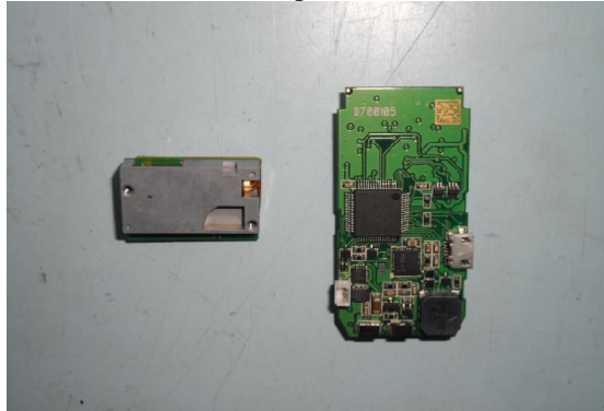
Inner Circuit Top View – All PCBs
