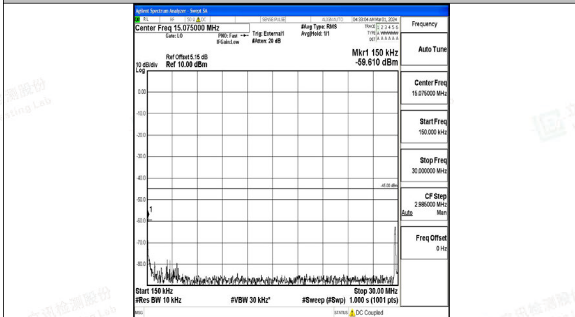
Band41_5MHz_16QAM_40620_1RB#0_0.15~30_0.15~30
