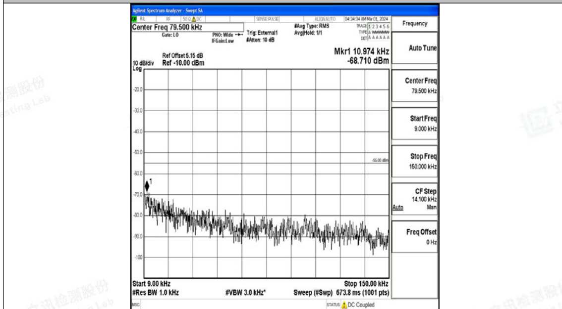
Band41_5MHz_QPSK_41565_1RB#0_0.009~0.15_0.009~0.15
