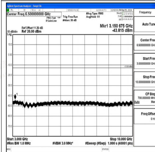
Band26_15MHz_QPSK_26915_1RB#0_3000~10000_000_3000~10000
