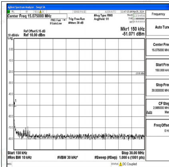
Band26_10MHz_16QAM_26990_1RB#0_0.15~3 0_0.15~30
