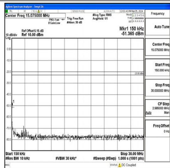
Band26_15MHz_QPSK_26915_1RB#0_0.15~30 0.15~30
