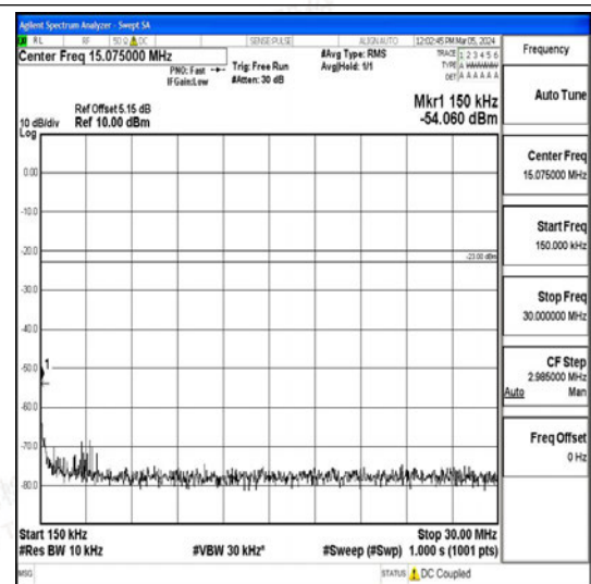
Band26_15MHz_QPSK_26965_1RB#0_0.15~30_0.15~30
