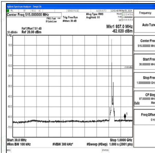
Band26_15MHz_QPSK_26915_1RB#0_30~1000_30~1000
