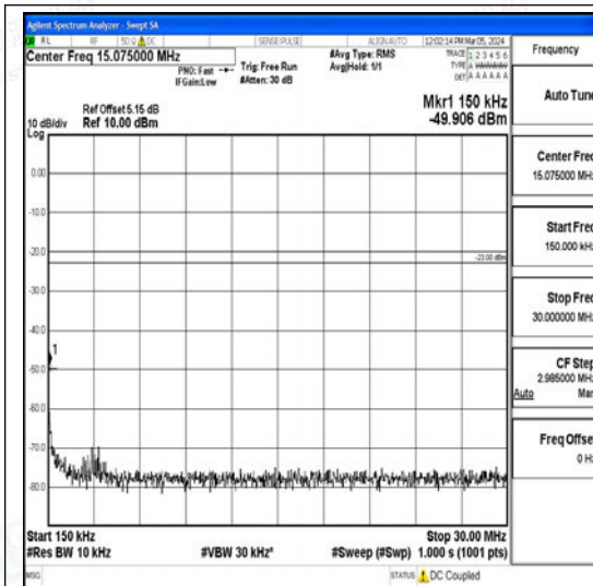
Band26_15MHz_16QAM_26915_1RB#0_0.15~3 0_0.15~30
