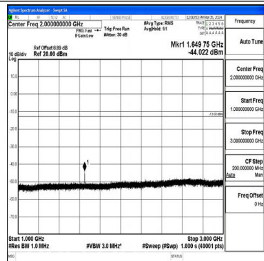
Band26_15MHz_QPSK_26865_1RB#0_1000~3000_0_1000~3000
