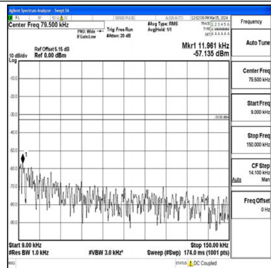
Band26_15MHz_16QAM_26915_1RB#0_0.009~0.15_0.009~0.15
