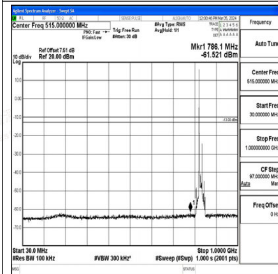
Band26_15MHz_QPSK_26865_1RB#0_30~1000_30~1000
