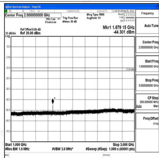
Band26_10MHz_QPSK_26990_1RB#0_1000~3000_0_1000~3000
