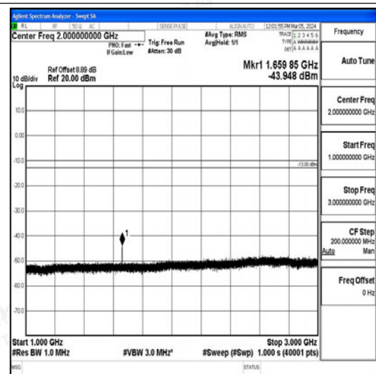
Band26_15MHz_QPSK_26915_1RB#0_1000~3000_0_1000~3000
