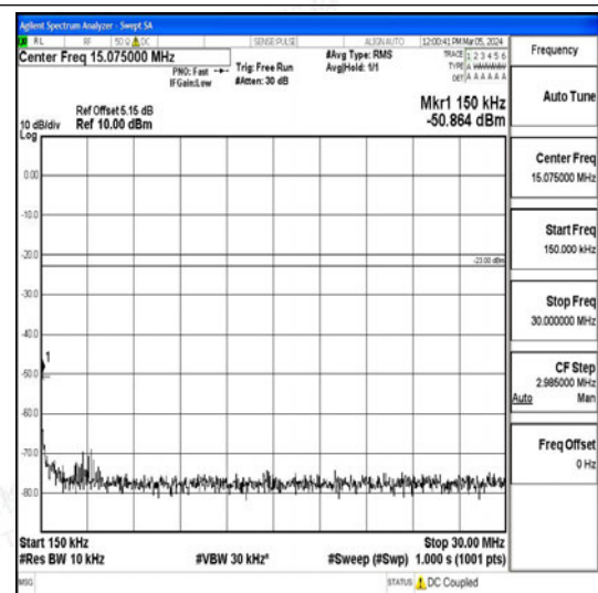
Band26_15MHz_QPSK_26865_1RB#0_0.15~30_0.15~30
