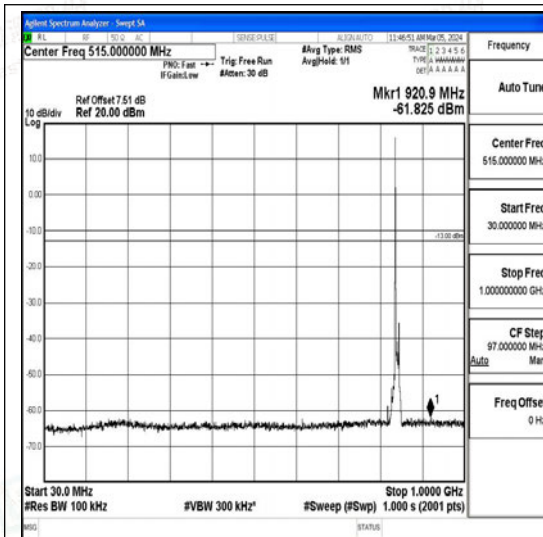
Band26_10MHz_QPSK_26990_1RB#0_30~1000_30~1000
