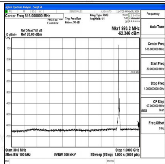
Band26_10MHz_16QAM_26990_1RB#0_30~1000 _30~1000
