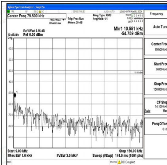
Band26_15MHz_QPSK_26965_1RB#0_0.009~0.15_0.009~0.15
