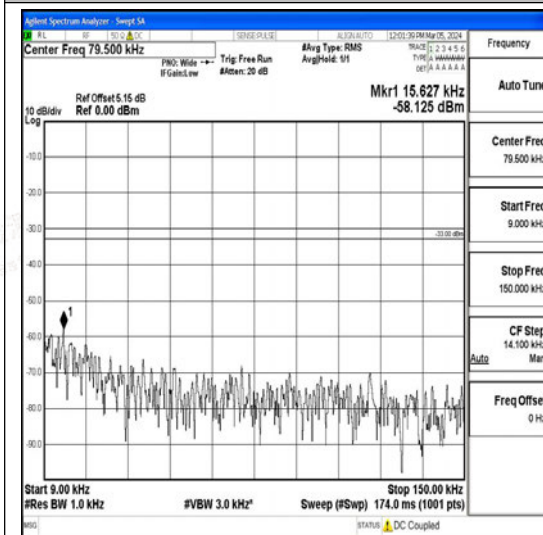
Band26_15MHz_QPSK_26915_1RB#0_0.009~0.15 15_0.009~0.15
