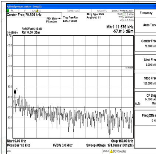
Band26_15MHz_QPSK_26865_1RB#0_0.009~0.15_0.009~0.15
