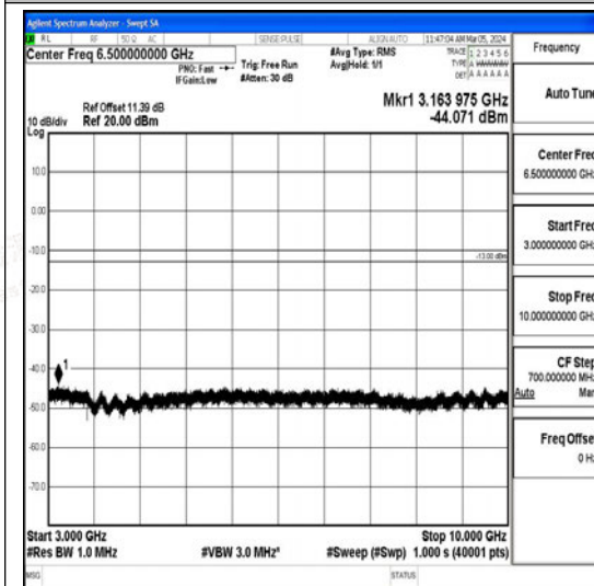
Band26_10MHz_QPSK_26990_1RB#0_3000~10000_000_3000~10000
