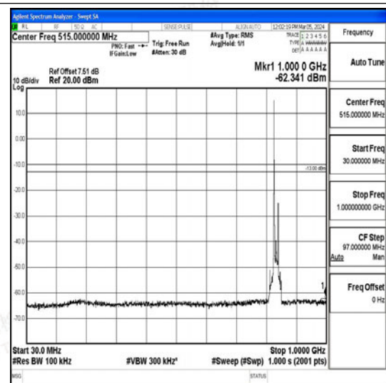
Band26_15MHz_16QAM_26915_1RB#0_30~1000 _30~1000
