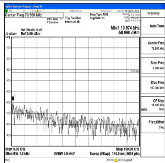
Band26_10MHz_16QAM_26990_1RB#0_0.009~0.15_0.009~0.15
