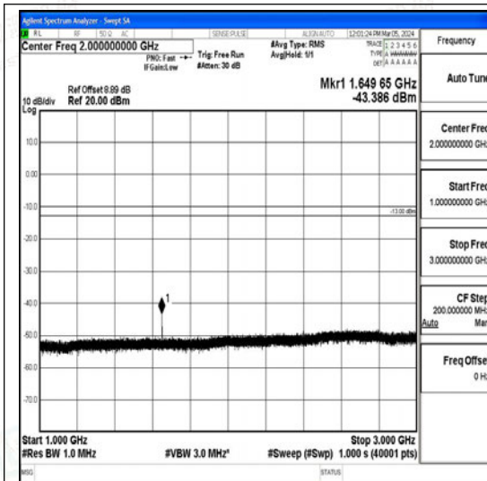
Band26_15MHz_16QAM_26865_1RB#0_1000~3000 000_1000~3000
