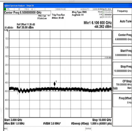
Band26_15MHz_16QAM_26865_1RB#0_3000~10000 000_3000~10000
