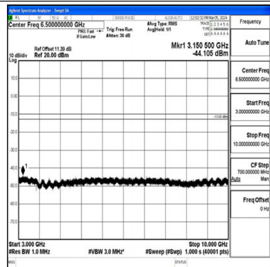
Band26_15MHz_16QAM_26915_1RB#0_3000~10 000_3000~10000
