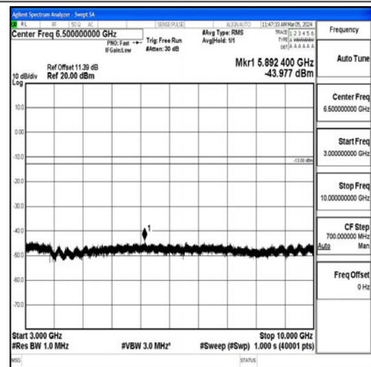
Band26_10MHz_16QAM_26990_1RB#0_3000~10 000_3000~10000
