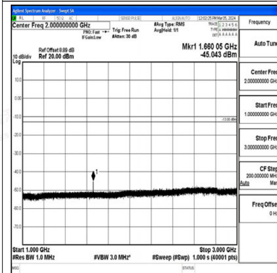
Band26_15MHz_16QAM_26915_1RB#0_1000~3 000_1000~3000
