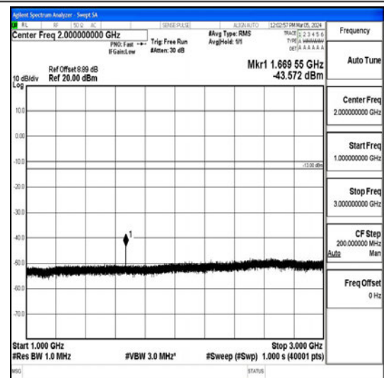
Band26_15MHz_QPSK_26965_1RB#0_1000~3000_0_1000~3000
