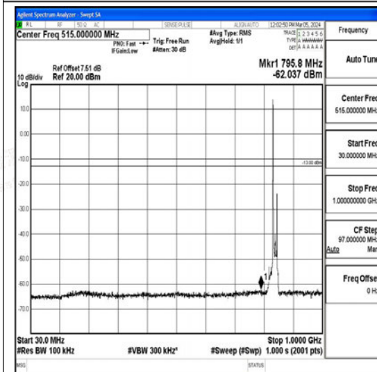
Band26_15MHz_QPSK_26965_1RB#0_30~1000_30~1000
