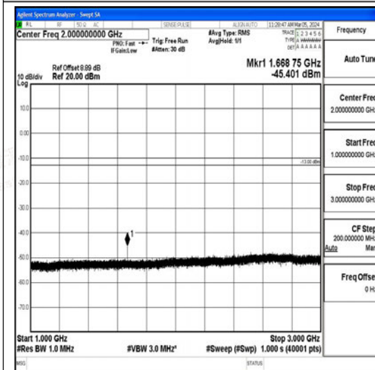
Band26_5MHz_16QAM_26915_1RB#0_1000~3000_00_1000~3000
