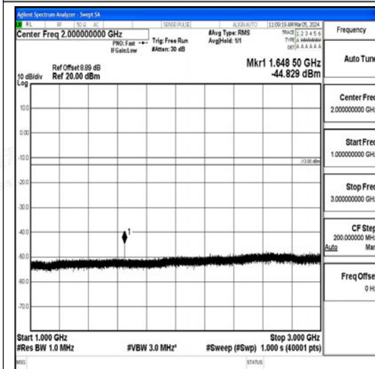
Band26_3MHz_16QAM_26805_1RB#0_1000~3000_1000~3000
