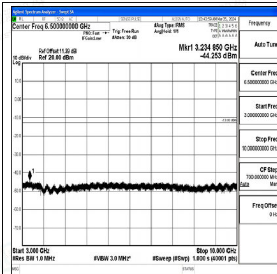
Band26_1.4MHz_QPSK_26797_1RB#0_3000~10000_3000~10000
