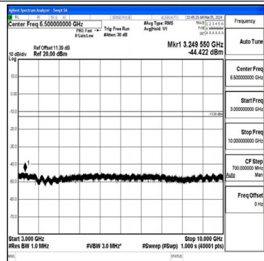
Band26_1.4MHz_16QAM_26915_1RB#0_3000~1 0000_3000~10000
