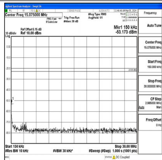
Band26_10MHz_QPSK_26990_1RB#0_0.15~30_0.15~30
