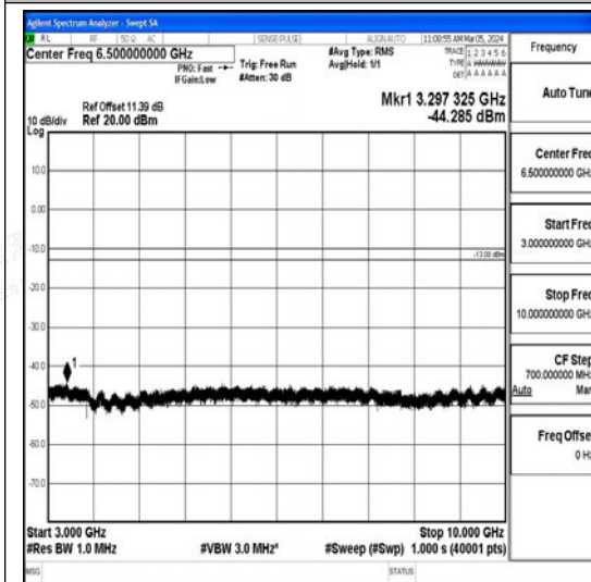
Band26_3MHz_QPSK_26805_1RB#0_3000~100_00_3000~10000
