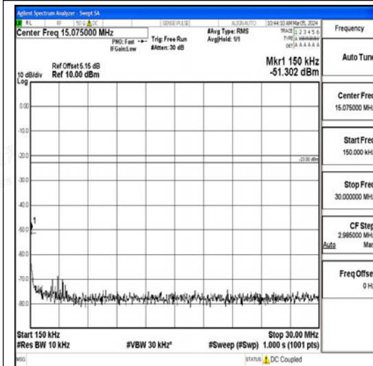
Band26_1.4MHz_16QAM_26797_1RB#0_0.15~30_0.15~30
