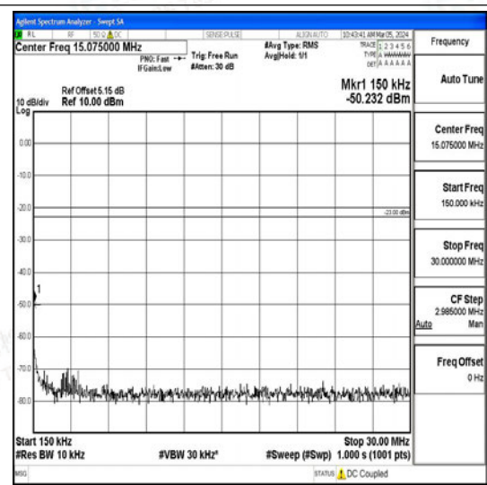
Band26_1.4MHz_QPSK_26797_1RB#0_0.15~30_0.15~30
