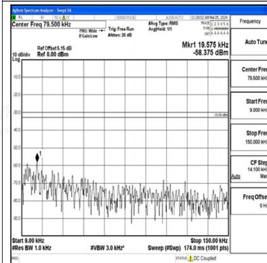
Band26_5MHz_QPSK_26915_1RB#0_0.009~0.1 5_0.009~0.15
