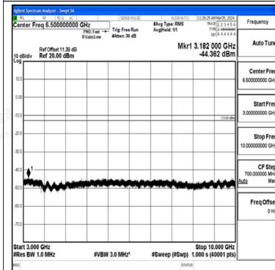
Band26_5MHz_QPSK_26915_1RB#0_3000~100_00_3000~10000
