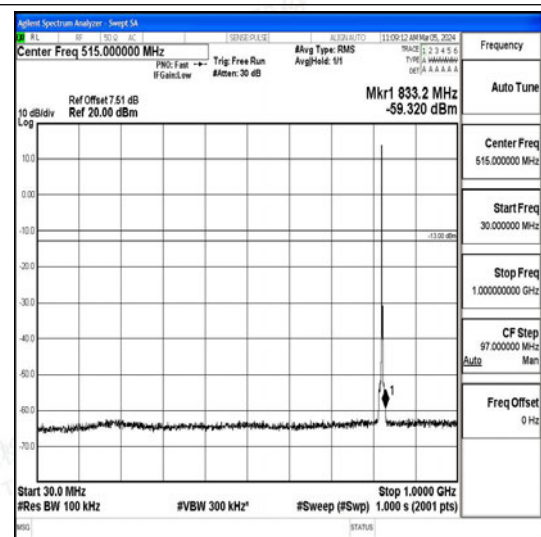
Band26_3MHz_16QAM_26805_1RB#0_30~1000_30~1000
