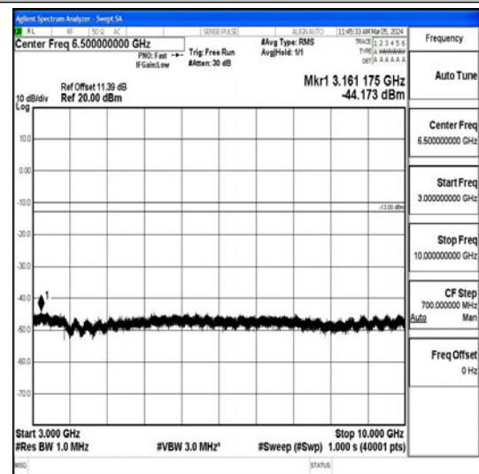
Band26_10MHz_16QAM_26840_1RB#0_3000~10 000_3000~10000
