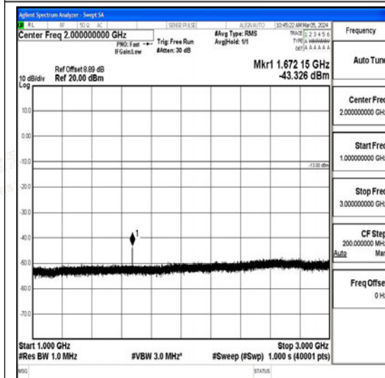
Band26_1.4MHz_16QAM_26915_1RB#0_1000~ 3000_1000~3000
