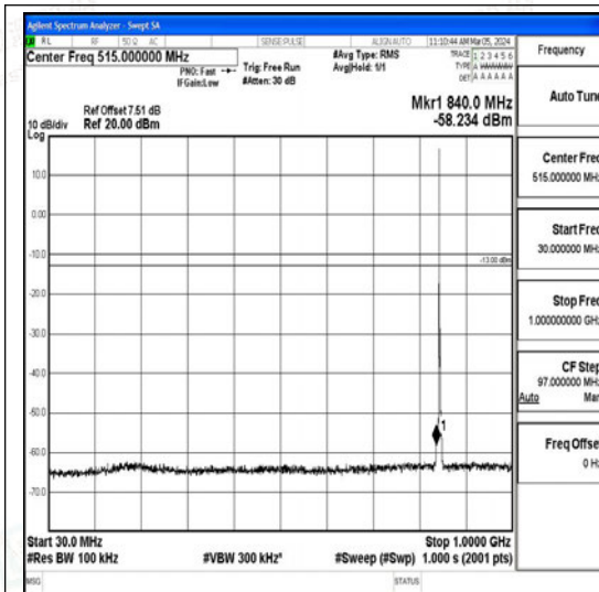
Band26_3MHz_QPSK_27025_1RB#0_30~1000_30~1000
