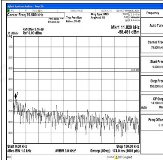
Band26_1.4MHz_QPSK_26915_1RB#0_0.009~0. 15_0.009~0.15
