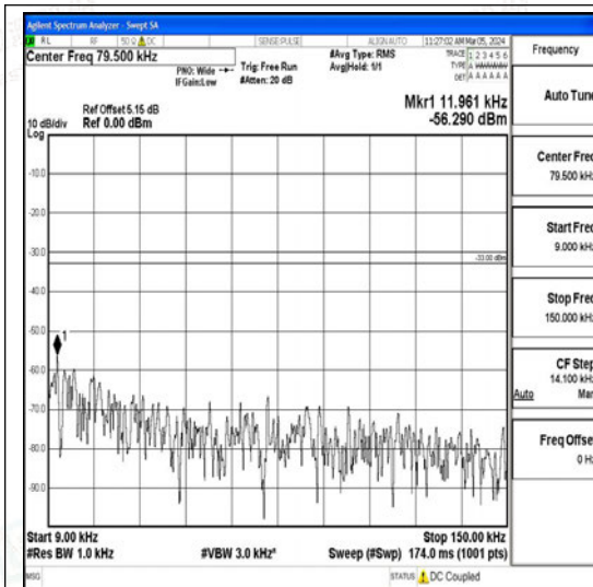
Band26_5MHz_QPSK_26815_1RB#0_0.009~0.15 5_0.009~0.15
