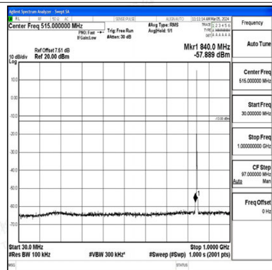
Band26_3MHz_16QAM_27025_1RB#0_30~1000_30~1000
