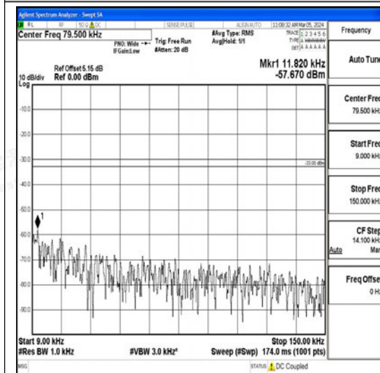
Band26_3MHz_QPSK_26805_1RB#0_0.009~0.1 5_0.009~0.15
