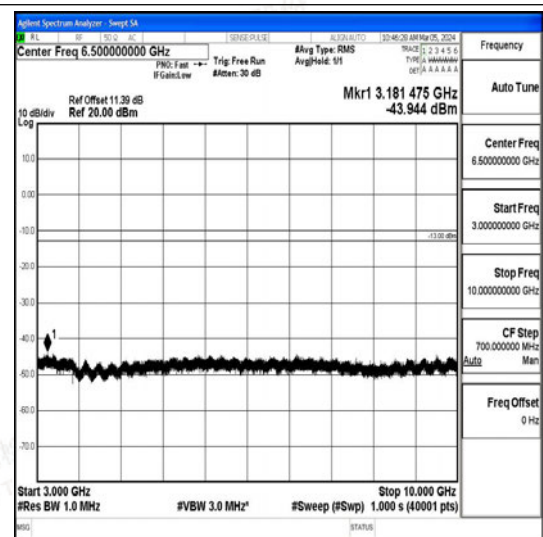
Band26_1.4MHz_16QAM_27033_1RB#0_3000~1 0000_3000~10000
