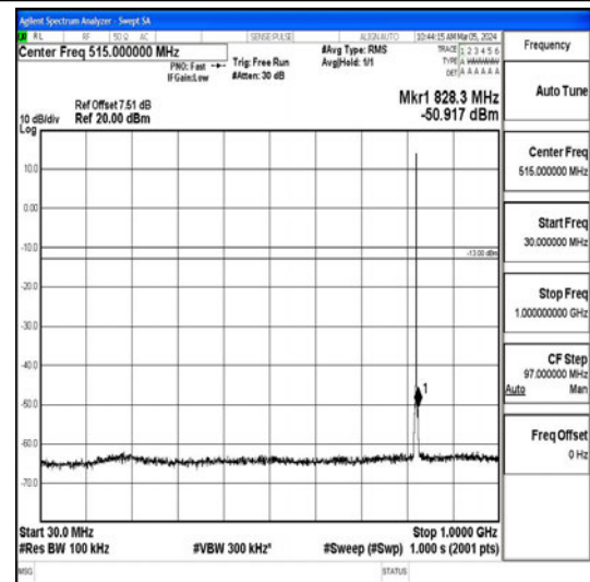
Band26_1.4MHz_16QAM_26797_1RB#0_0_30~1000_0_30~1000
