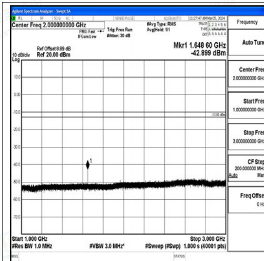
Band26_5MHz_16QAM_26815_1RB#0_1000~3000 00_1000~3000
