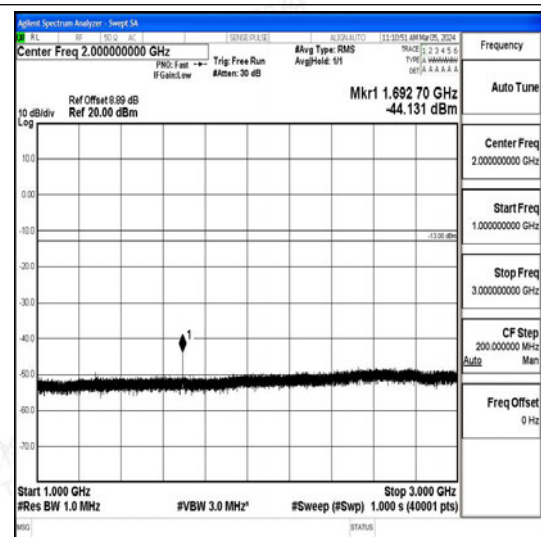
Band26_3MHz_QPSK_27025_1RB#0_1000~3000_1000~3000
