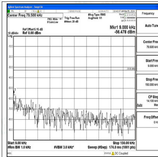
Band26_1.4MHz_QPSK_26797_1RB#0_0.009~0.15_0.009~0.15
