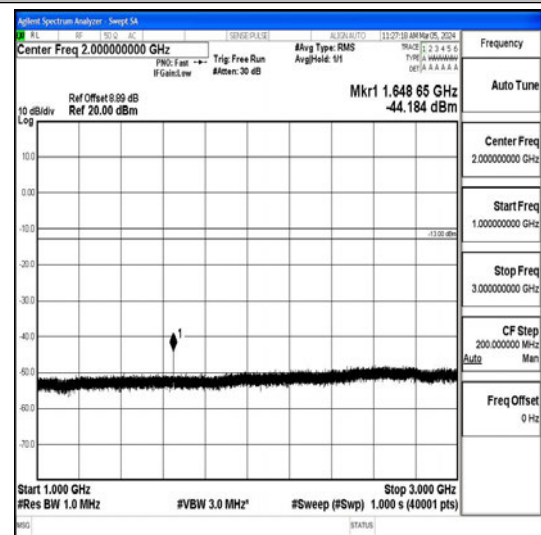
Band26_5MHz_QPSK_26815_1RB#0_1000~3000_1000~3000
