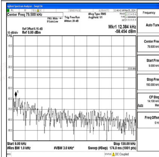
Band26_10MHz_QPSK_26990_1RB#0_0.009~0.15_0.009~0.15
