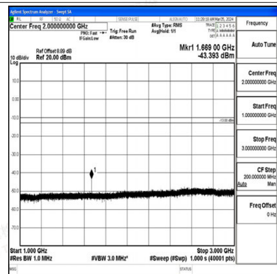
Band26_5MHz_QPSK_26915_1RB#0_1000~3000_1000~3000
