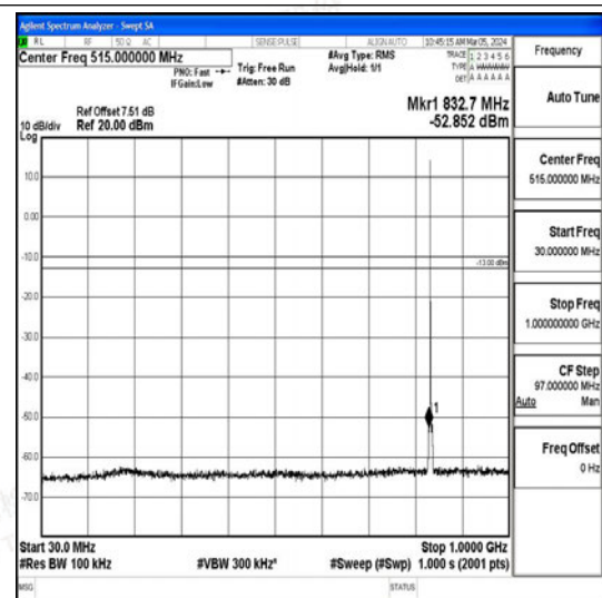
Band26_1.4MHz_16QAM_26915_1RB#0_30~100 0_30~1000
