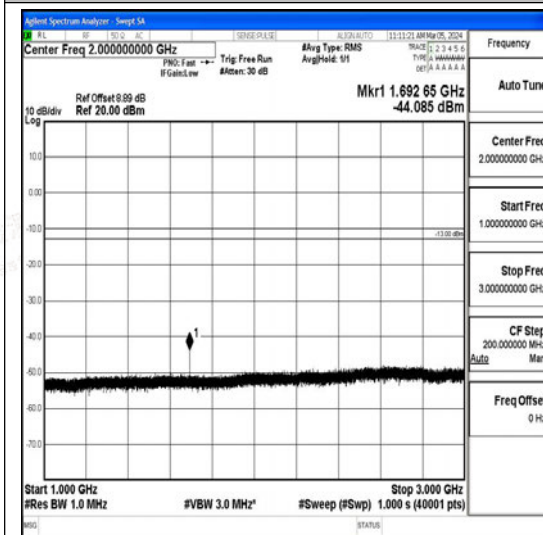
Band26_3MHz_16QAM_27025_1RB#0_1000~3000_00_1000~3000
