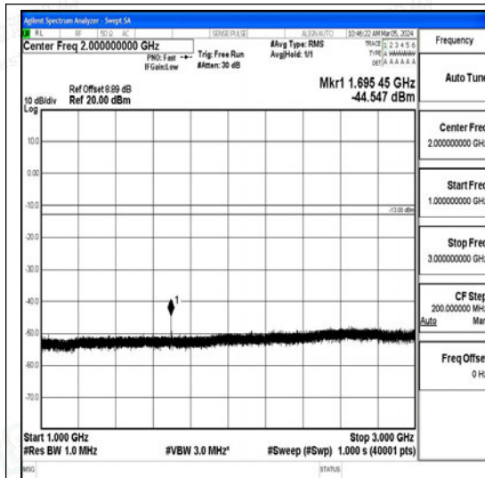
Band26_1.4MHz_16QAM_27033_1RB#0_1000~ 3000_1000~3000
