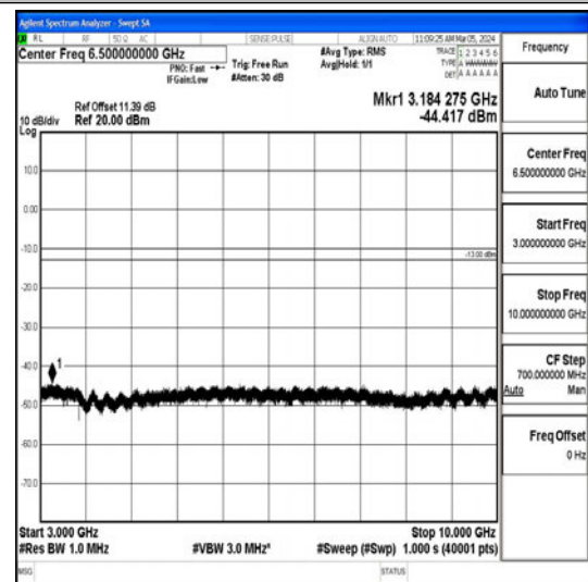
Band26_3MHz_16QAM_26805_1RB#0_3000~10000_3000~10000
