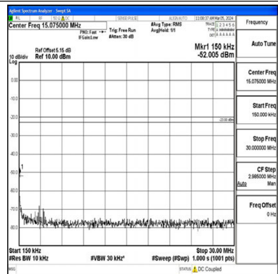
Band26_3MHz_QPSK_26805_1RB#0_0.15~30_0. 15~30
