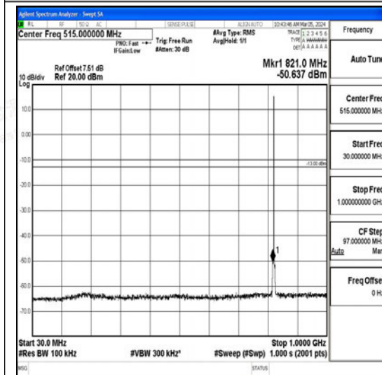
Band26_1.4MHz_QPSK_26797_1RB#0_30~1000_30~1000
