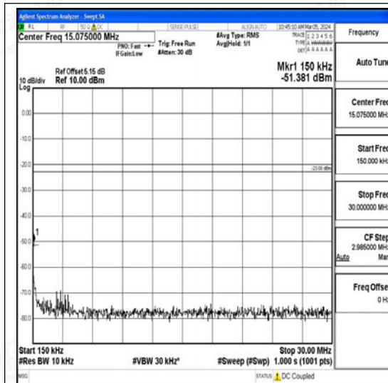
Band26_1.4MHz_16QAM_26915_1RB#0_0.15~30 0_0.15~30
