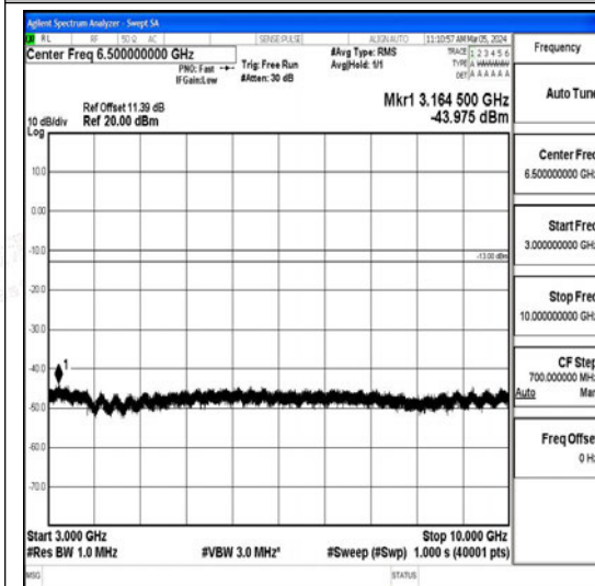
Band26_3MHz_QPSK_27025_1RB#0_3000~10000_3000~10000
