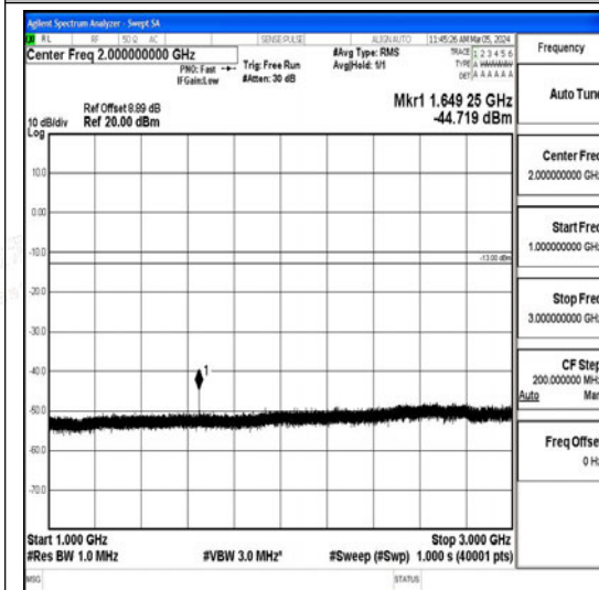
Band26_10MHz_16QAM_26840_1RB#0_1000~3 000_1000~3000
