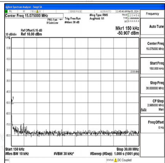
Band26_10MHz_QPSK_26915_1RB#0_0.15~30_0.15~30
