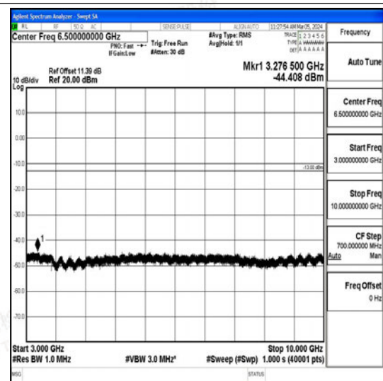
Band26_5MHz_16QAM_26815_1RB#0_3000~10000 00_3000~10000
