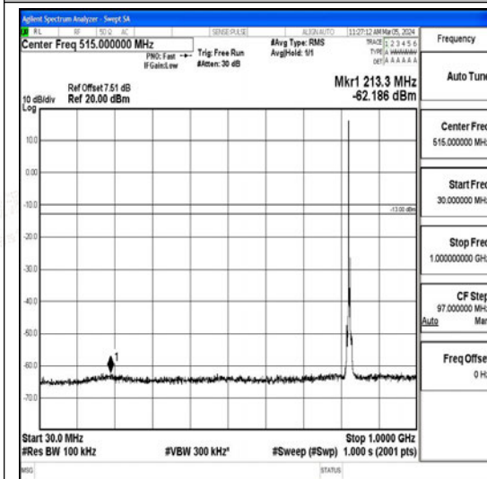
Band26_5MHz_QPSK_26815_1RB#0_30~1000_30~1000
