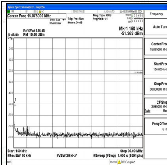
Band26_10MHz_16QAM_26840_1RB#0_0.15~3 0_0.15~30
