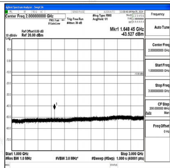
Band26_3MHz_QPSK_26805_1RB#0_1000~3000_1000~3000
