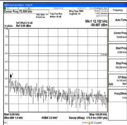
Band26_3MHz_16QAM_27025_1RB#0_0.009~0.15_5_0.009~0.15
