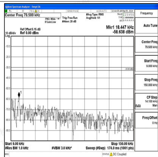
Band26_1.4MHz_16QAM_26797_1RB#0_0.009~0.15_0.009~0.15
