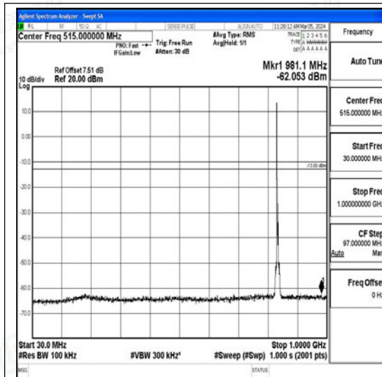
Band26_5MHz_QPSK_26915_1RB#0_30~1000_30~1000
