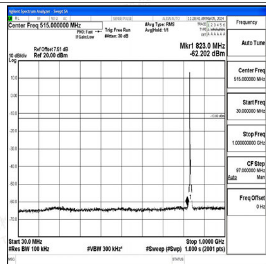
Band26_5MHz_16QAM_26915_1RB#0_30~1000_30~1000
