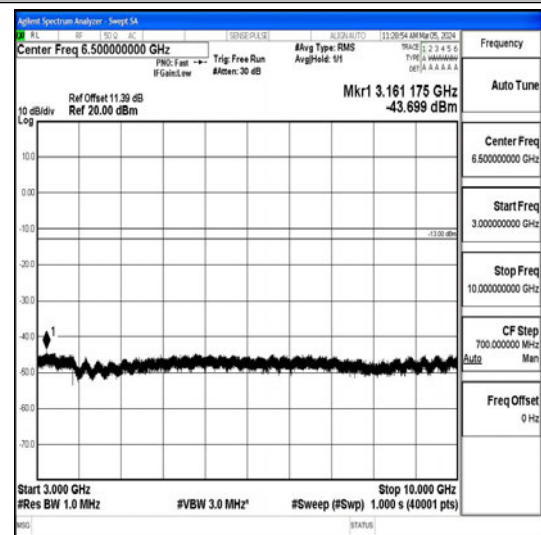
Band26_5MHz_16QAM_26915_1RB#0_3000~10000_00_3000~10000
