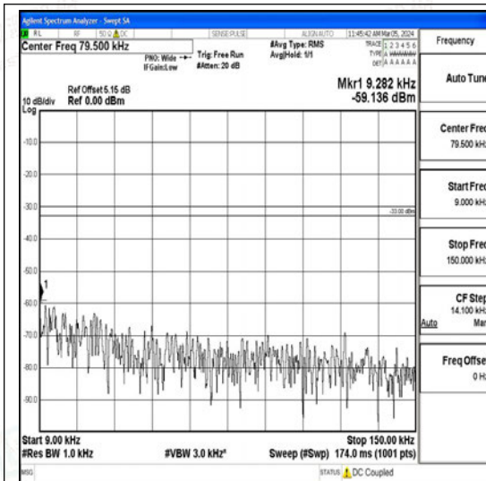
Band26_10MHz_QPSK_26915_1RB#0_0.009~0.15_0.009~0.15
