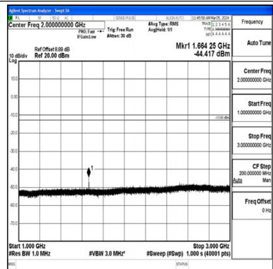
Band26_10MHz_QPSK_26915_1RB#0_1000~3000_0_1000~3000
