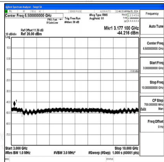
Band26_10MHz_16QAM_26915_1RB#0_3000~10000_3000~10000
