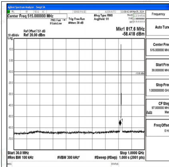
Band26_3MHz_QPSK_26805_1RB#0_30~1000_30~1000
