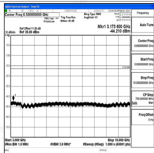
Band26_1.4MHz_16QAM_26797_1RB#0_3000~1 0000_3000~10000
