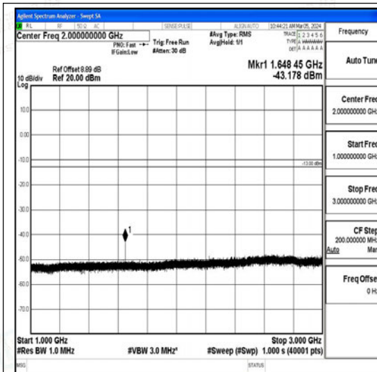
Band26_1.4MHz_16QAM_26797_1RB#0_1000~ 3000_1000~3000
