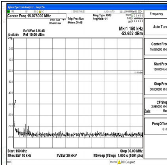
Band26_3MHz_16QAM_27025_1RB#0_0.15~30_0.15~30
