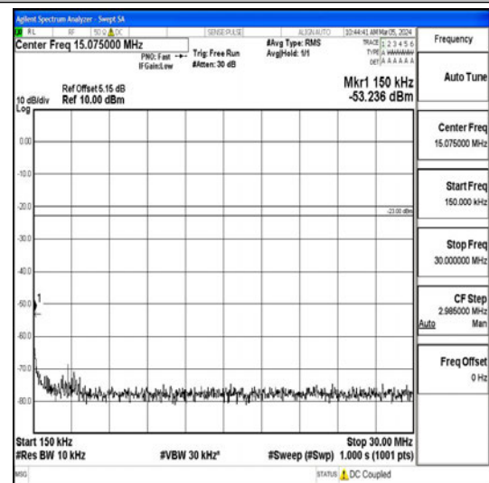
Band26_1.4MHz_QPSK_26915_1RB#0_0.15~30_ 0.15~30
