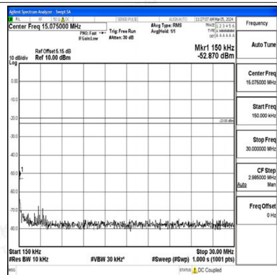
Band26_5MHz_QPSK_26815_1RB#0_0.15~30_0. 15~30
