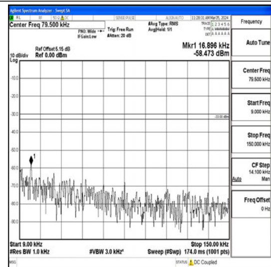
Band26_5MHz_16QAM_26915_1RB#0_0.009~0.15_5_0.009~0.15
