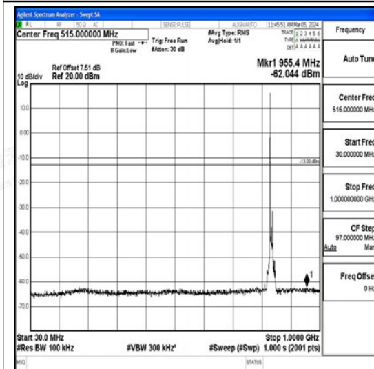
Band26_10MHz_QPSK_26915_1RB#0_30~1000_30~1000
