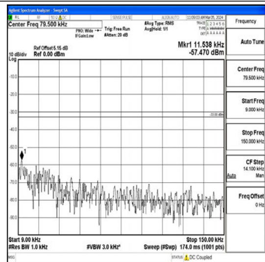
Band26_3MHz_16QAM_26805_1RB#0_0.009~0.15_5_0.009~0.15
