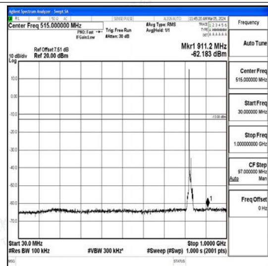
Band26_10MHz_16QAM_26840_1RB#0_30~1000 _30~1000
