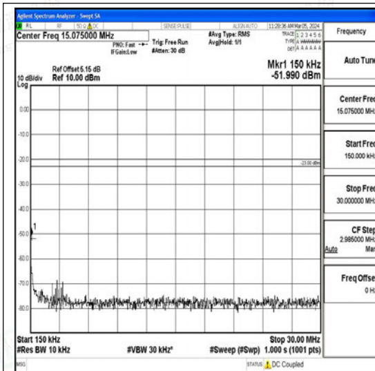
Band26_5MHz_16QAM_26915_1RB#0_0.15~30_0.15~30
