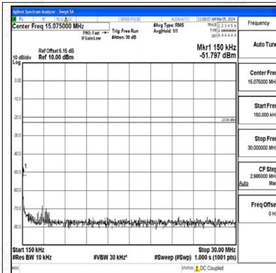
Band26_3MHz_16QAM_26805_1RB#0_0.15~30_0.15~30
