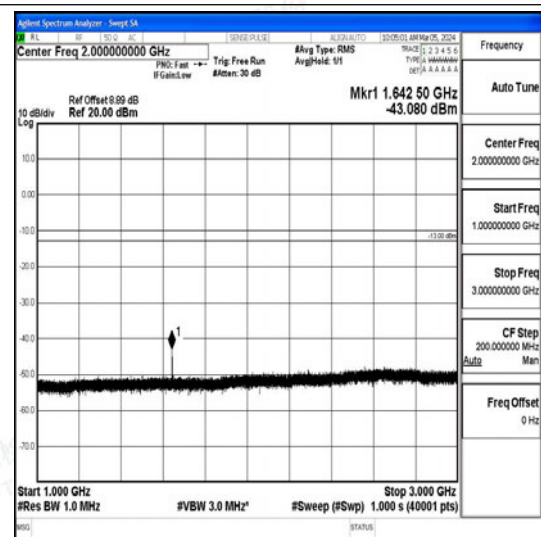
Band26_3MHz_QPSK_26775_1RB#0_1000~3000_1000~3000
