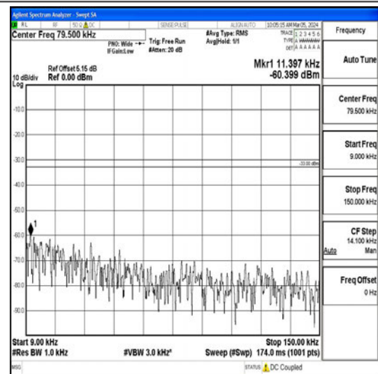
Band26_3MHz_16QAM_26775_1RB#0_0.009~0.15_5_0.009~0.15
