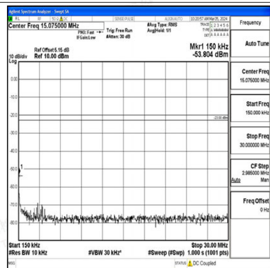
Band26_5MHz_QPSK_26715_1RB#0_0.15~30_0. 15~30
