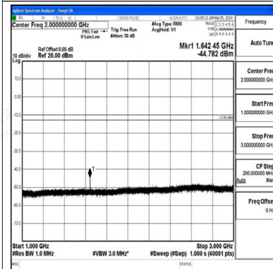
Band26_3MHz_16QAM_26775_1RB#0_1000~3000_1000~3000
