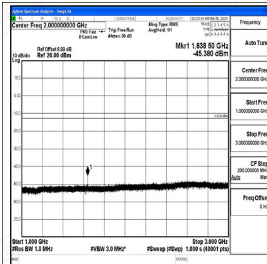
Band26_5MHz_16QAM_26765_1RB#0_1000~3000 00_1000~3000
