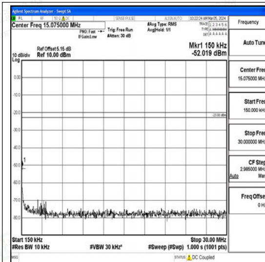
Band26_5MHz_16QAM_26740_1RB#0_0.15~30_0.15~30
