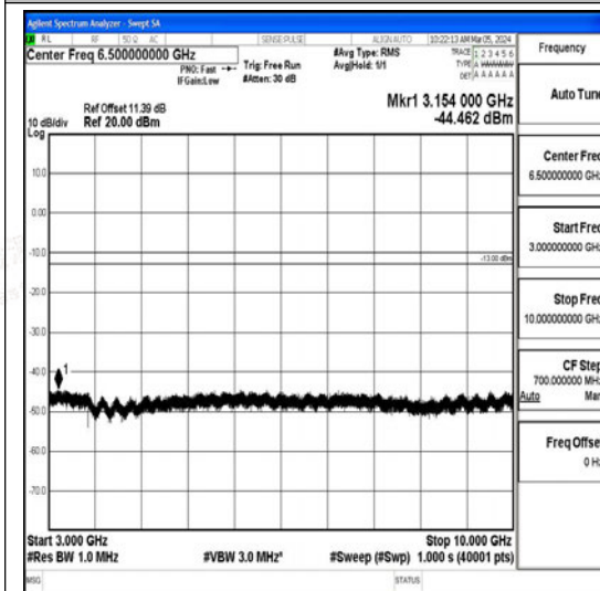
Band26_5MHz_QPSK_26740_1RB#0_3000~100_00_3000~10000
