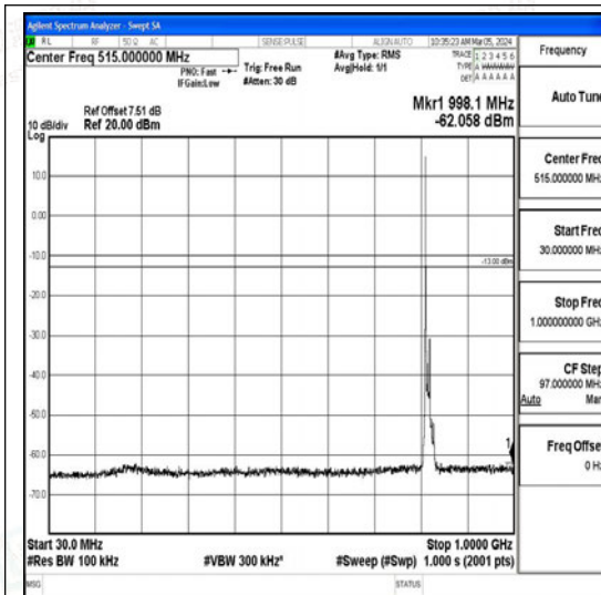
Band26_10MHz_QPSK_26740_1RB#0_30~1000_30~1000
