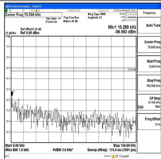
Band26_10MHz_16QAM_26740_1RB#0_0.009~0.15_0.009~0.15
