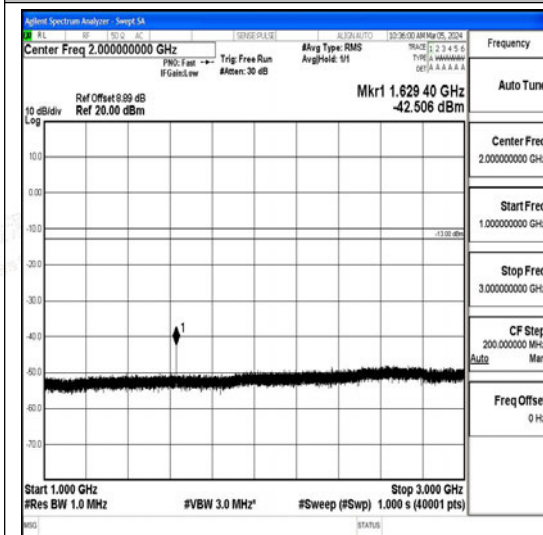
Band26_10MHz_16QAM_26740_1RB#0_1000~3 000_1000~3000
