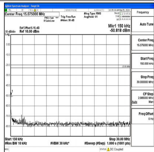
Band26_10MHz_QPSK_26740_1RB#0_0.15~30 0.15~30
