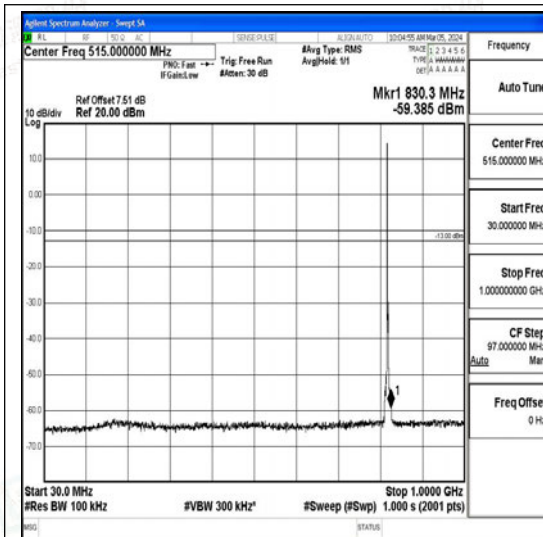
Band26_3MHz_QPSK_26775_1RB#0_30~1000_30~1000
