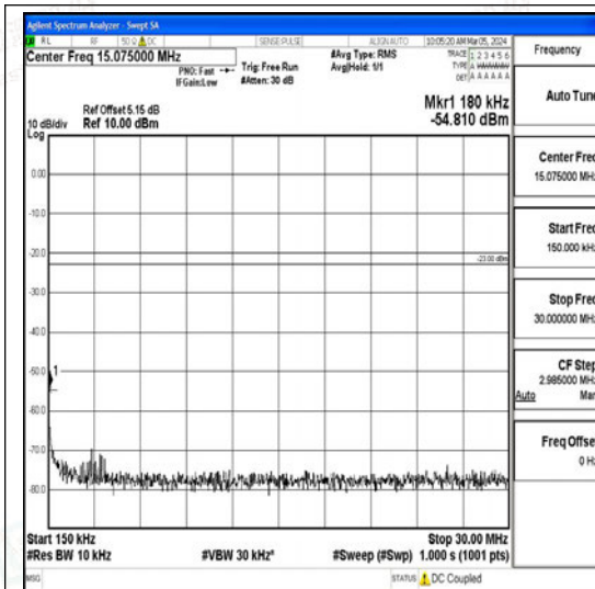
Band26_3MHz_16QAM_26775_1RB#0_0.15~30_0.15~30
