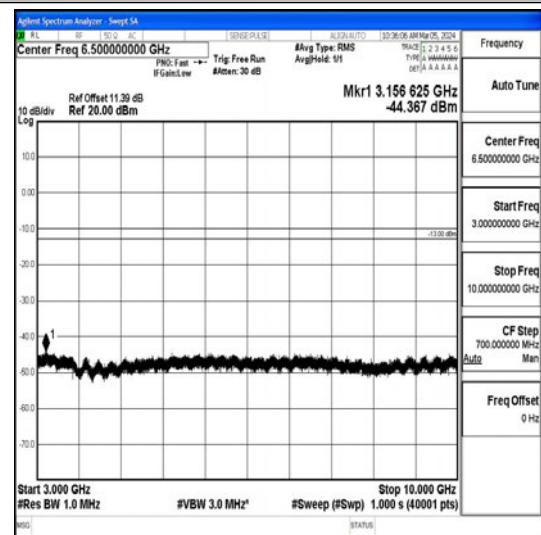
Band26_10MHz_16QAM_26740_1RB#0_3000~10 000_3000~10000
