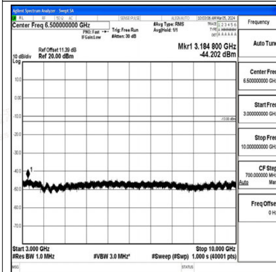
Band26_3MHz_QPSK_26705_1RB#0_3000~100_00_3000~10000
