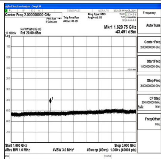
Band26_5MHz_QPSK_26715_1RB#0_1000~3000_1000~3000
