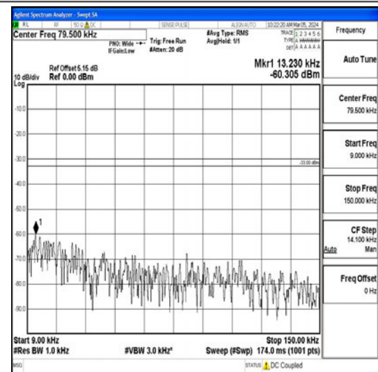
Band26_5MHz_16QAM_26740_1RB#0_0.009~0.15_5_0.009~0.15
