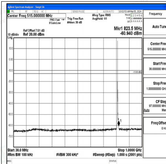
Band26_3MHz_QPSK_26705_1RB#0_30~1000_30~1000
