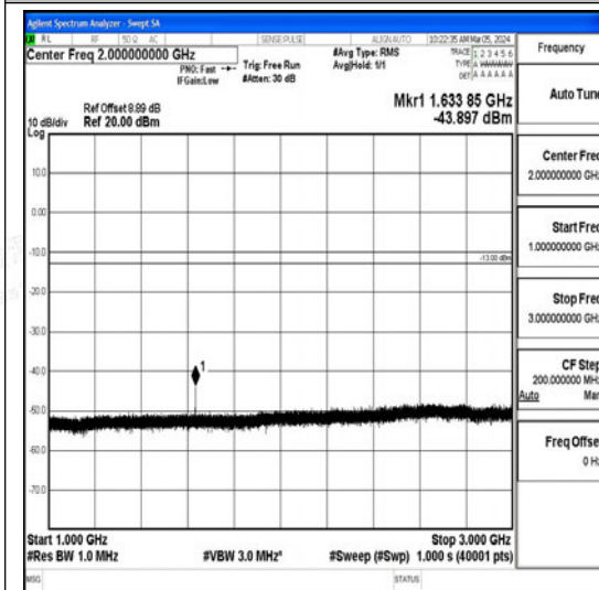
Band26_5MHz_16QAM_26740_1RB#0_1000~3000_00_1000~3000
