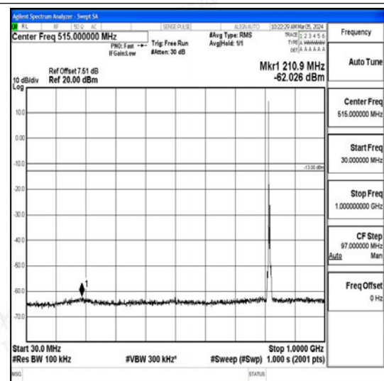
Band26_5MHz_16QAM_26740_1RB#0_30~1000_30~1000
