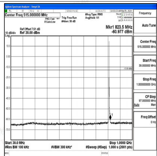
Band26_3MHz_16QAM_26705_1RB#0_30~1000_30~1000
