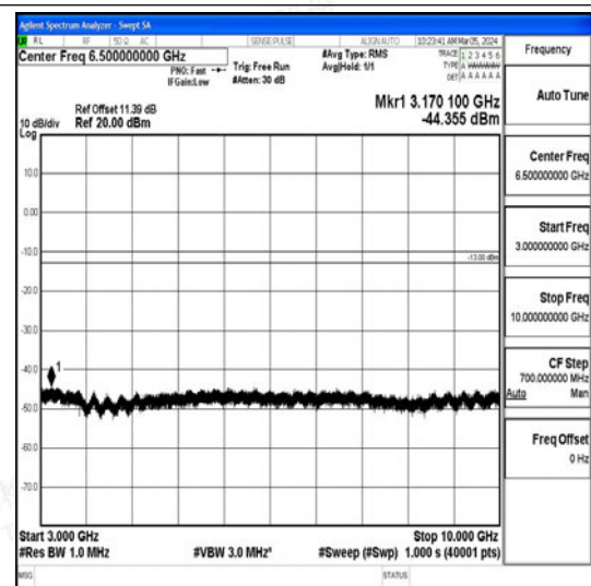
Band26_5MHz_16QAM_26765_1RB#0_3000~10000 00_3000~10000
