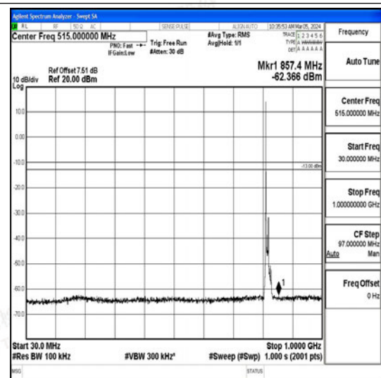
Band26_10MHz_16QAM_26740_1RB#0_30~1000 _30~1000
