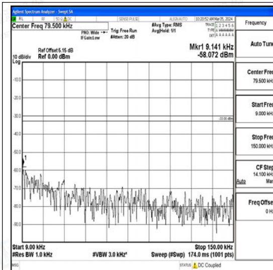
Band26_5MHz_QPSK_26715_1RB#0_0.009~0.15 5_0.009~0.15
