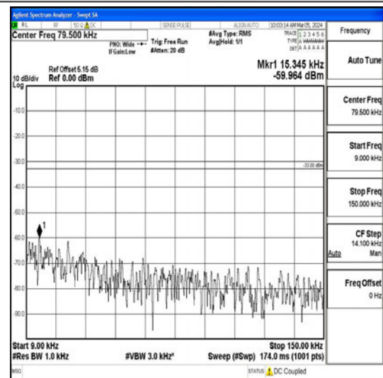
Band26_3MHz_16QAM_26705_1RB#0_0.009~0.15_5_0.009~0.15
