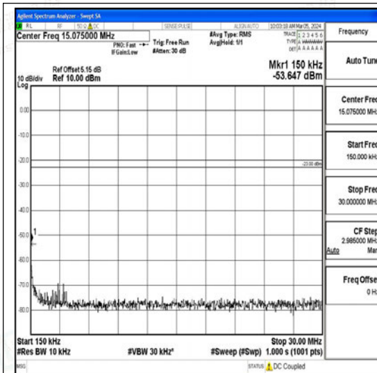
Band26_3MHz_16QAM_26705_1RB#0_0.15~30_0.15~30
