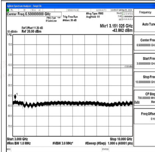
Band26_3MHz_QPSK_26775_1RB#0_3000~100_00_3000~10000
