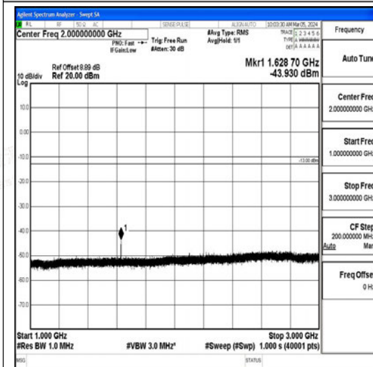
Band26_3MHz_16QAM_26705_1RB#0_1000~3000_1000~3000
