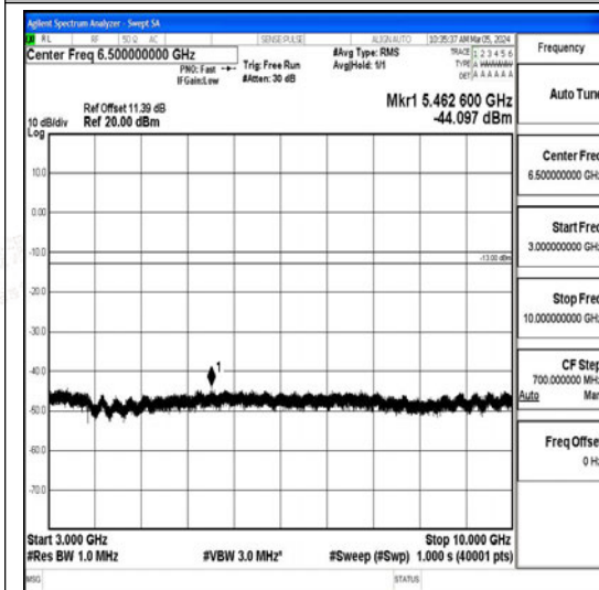
Band26_10MHz_QPSK_26740_1RB#0_3000~10000_000_3000~10000
