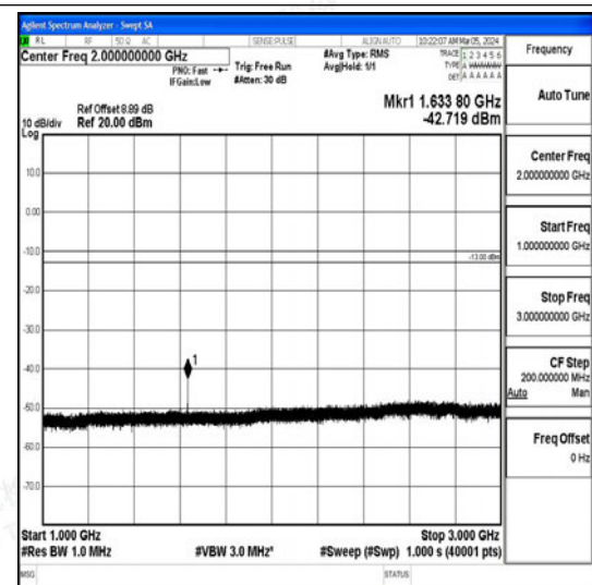
Band26_5MHz_QPSK_26740_1RB#0_1000~3000_1000~3000
