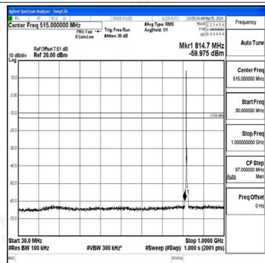
Band26_3MHz_16QAM_26775_1RB#0_30~1000_30~1000
