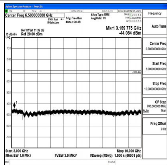
Band26_5MHz_16QAM_26740_1RB#0_3000~10000_00_3000~10000
