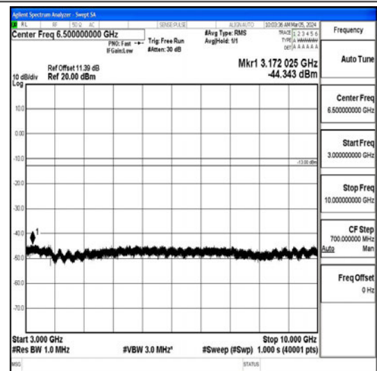
Band26_3MHz_16QAM_26705_1RB#0_3000~10000_3000~10000
