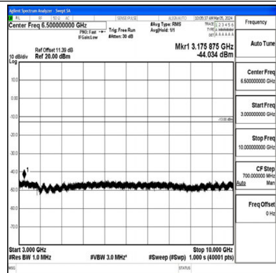
Band26_3MHz_16QAM_26775_1RB#0_3000~10000_3000~10000
