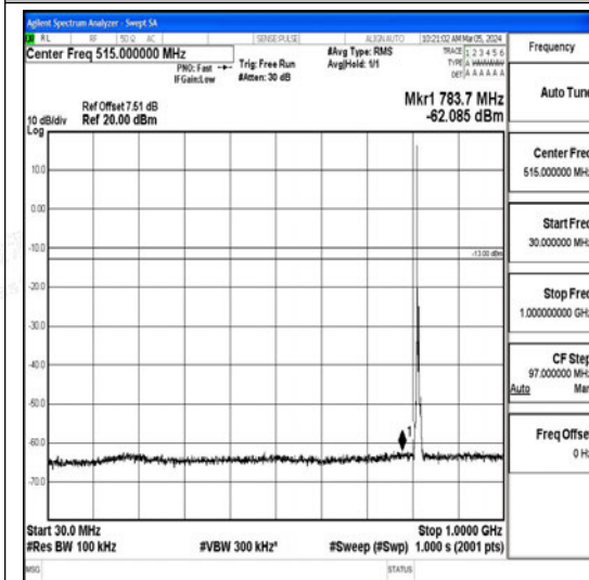
Band26_5MHz_QPSK_26715_1RB#0_30~1000_30~1000
