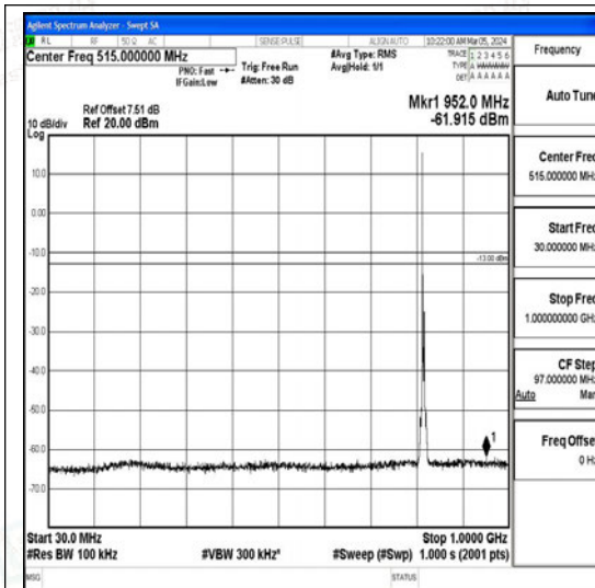
Band26_5MHz_QPSK_26740_1RB#0_30~1000_30~1000
