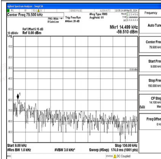
Band26_10MHz_QPSK_26740_1RB#0_0.009~0.15 15_0.009~0.15
