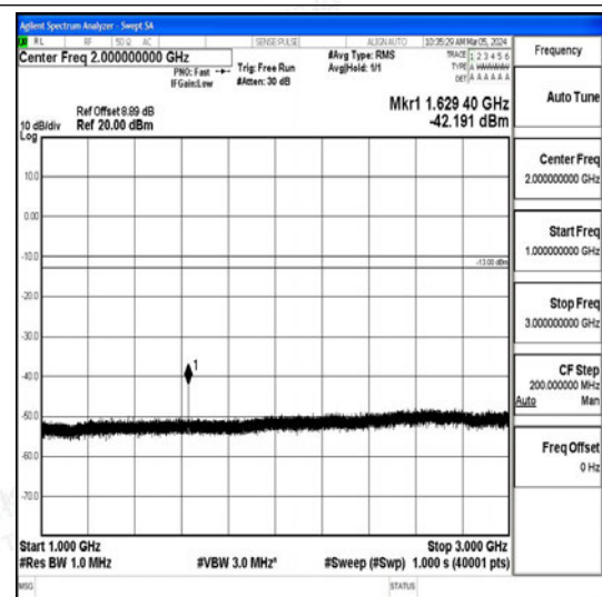
Band26_10MHz_QPSK_26740_1RB#0_1000~3000_0_1000~3000
