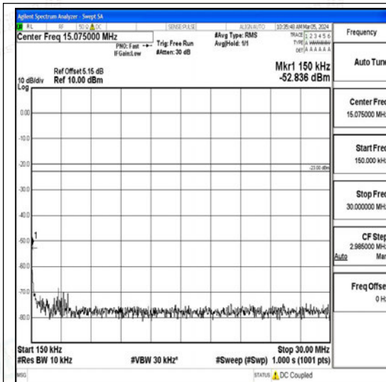
Band26_10MHz_16QAM_26740_1RB#0_0.15~30 0_0.15~30
