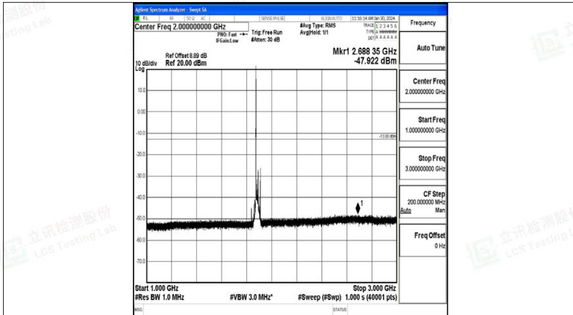
Band25_20MHz_16QAM_26365_1RB#0_1000~3000_1000~3000
