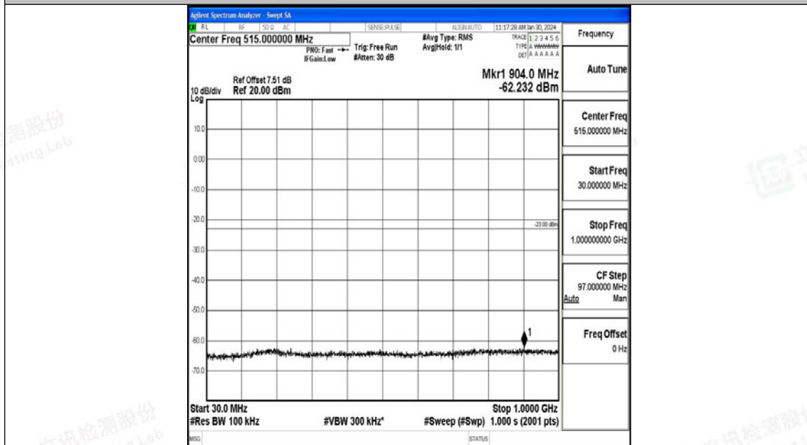
Band25_20MHz_16QAM_26590_1RB#0_30~1000_30~1000
