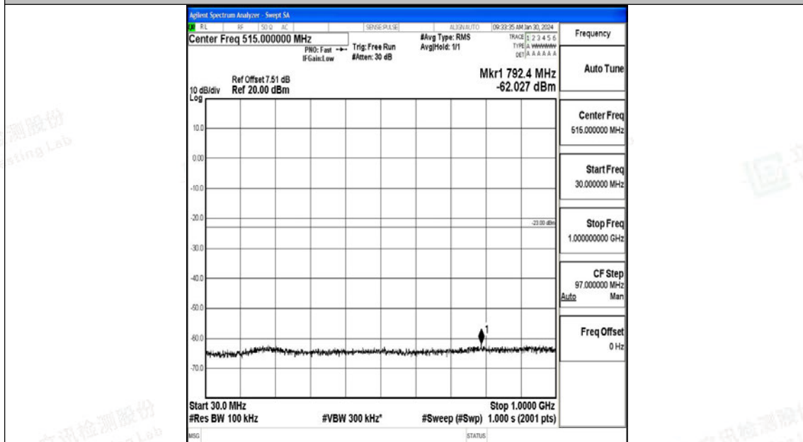
Band25_1.4MHz_16QAM_26365_1RB#0_30~1000_30~1000
