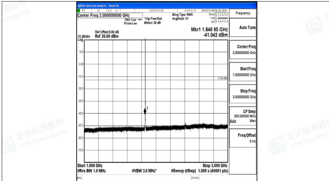
Band25_1.4MHz_16QAM_26047_1RB#0_1000~3000_1000~3000
