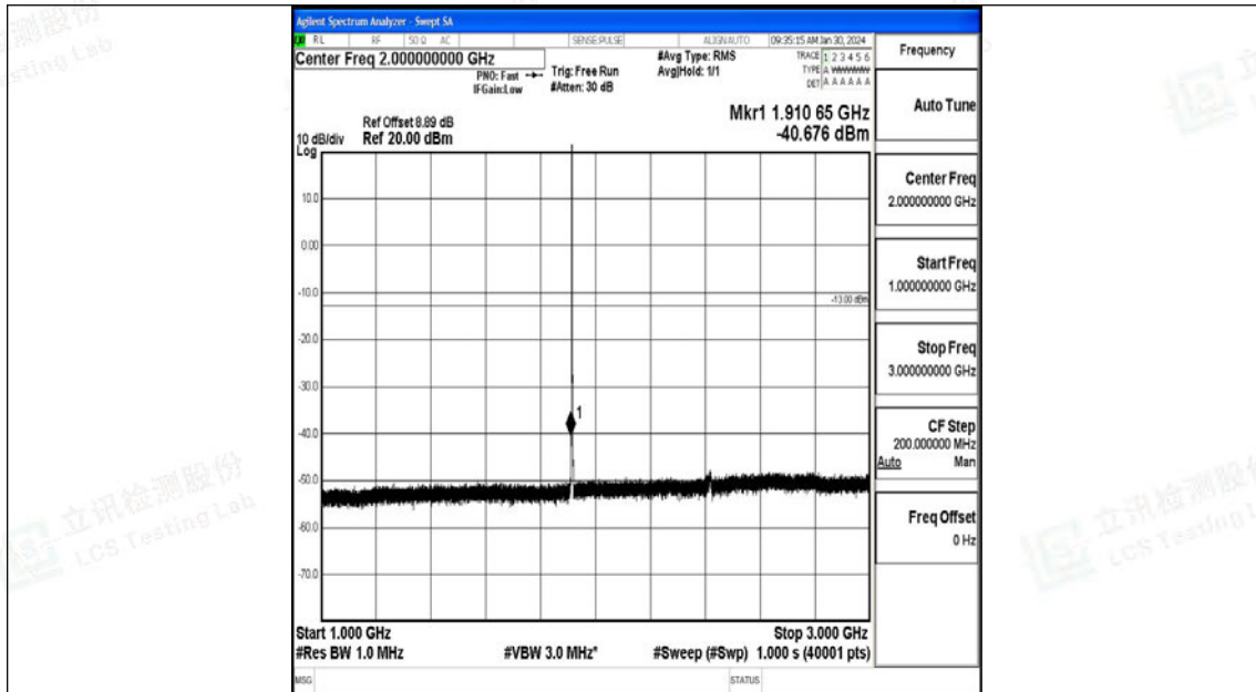
Band25_1.4MHz_16QAM_26683_1RB#0_1000~3000_1000~3000
