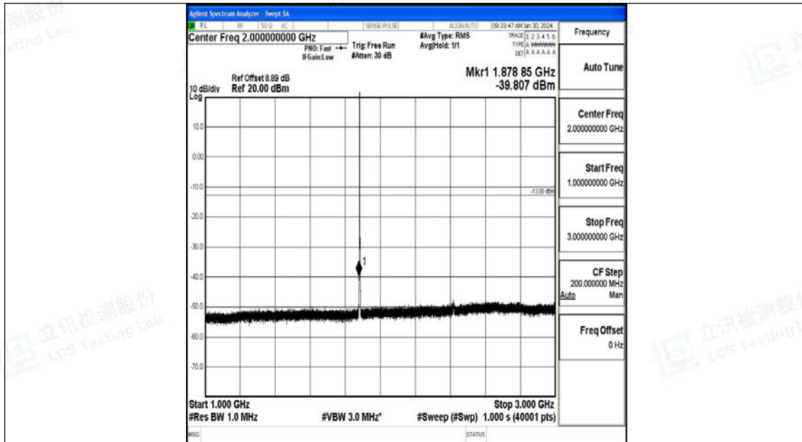
Band25_1.4MHz_16QAM_26365_1RB#0_1000~3000_1000~3000
