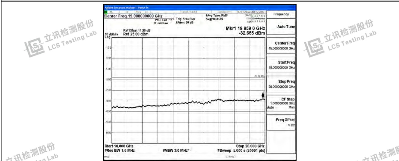
Band25-10MHz-QPSK-26365-1RB#0-Range1:0.009~0.15MHz
