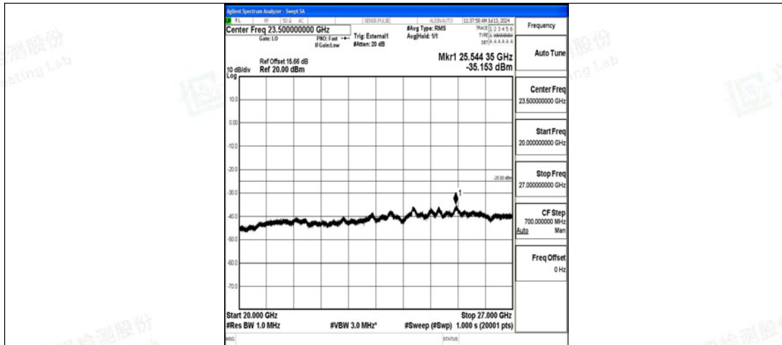
Band41_5MHz_QPSK_41565_1RB#0_20000~27000_20000~27000
