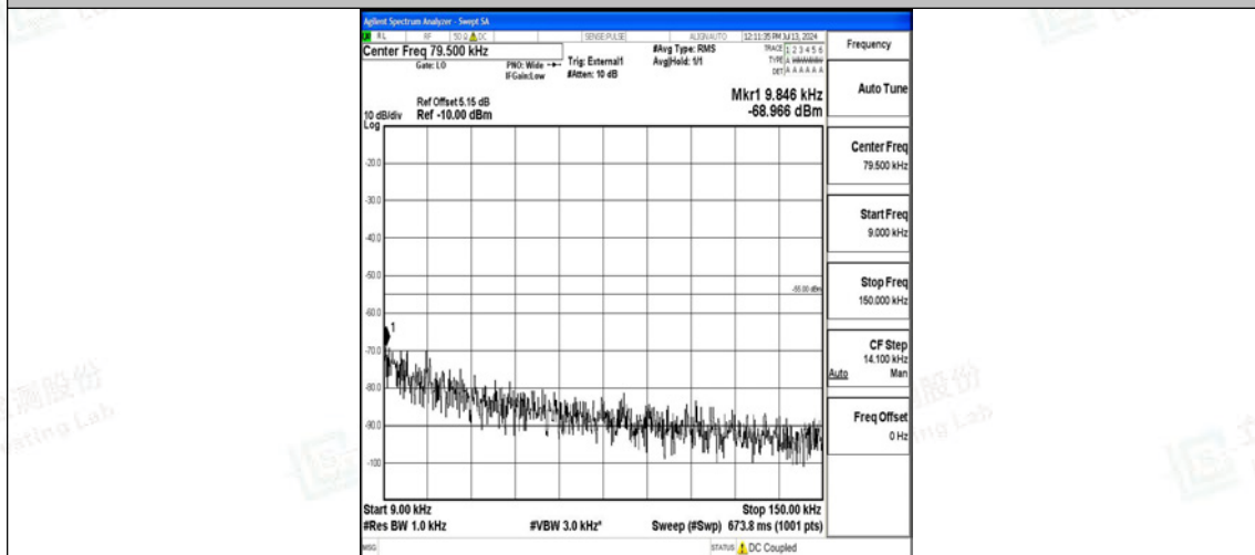
Band41_10MHz_16QAM_41540_1RB#0_0.009~0.15_0.009~0.15
