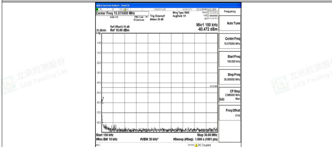
Band41_10MHz_16QAM_41540_1RB#0_0.15~30_0.15~30
