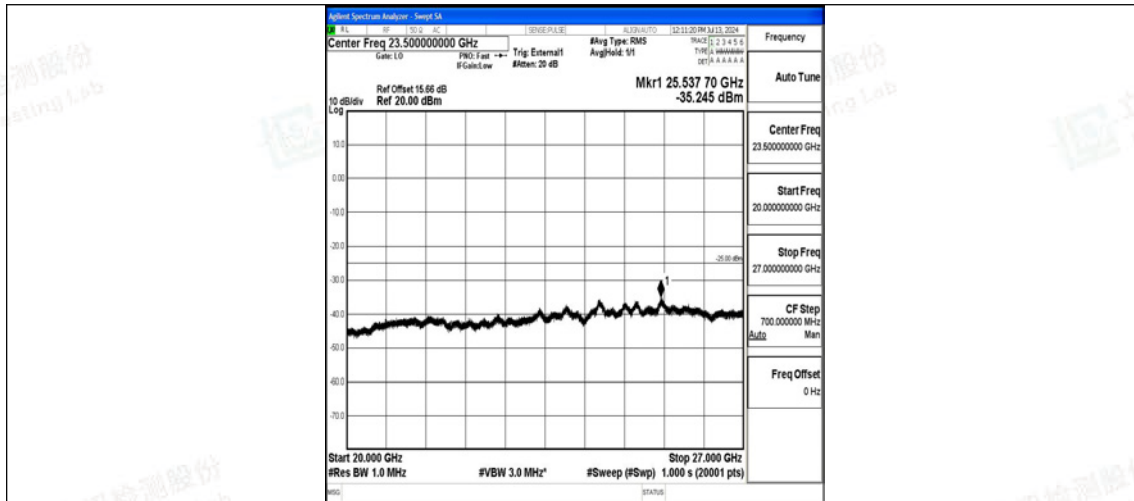
Band41_10MHz_QPSK_41540_1RB#0_20000~27000_20000~27000
