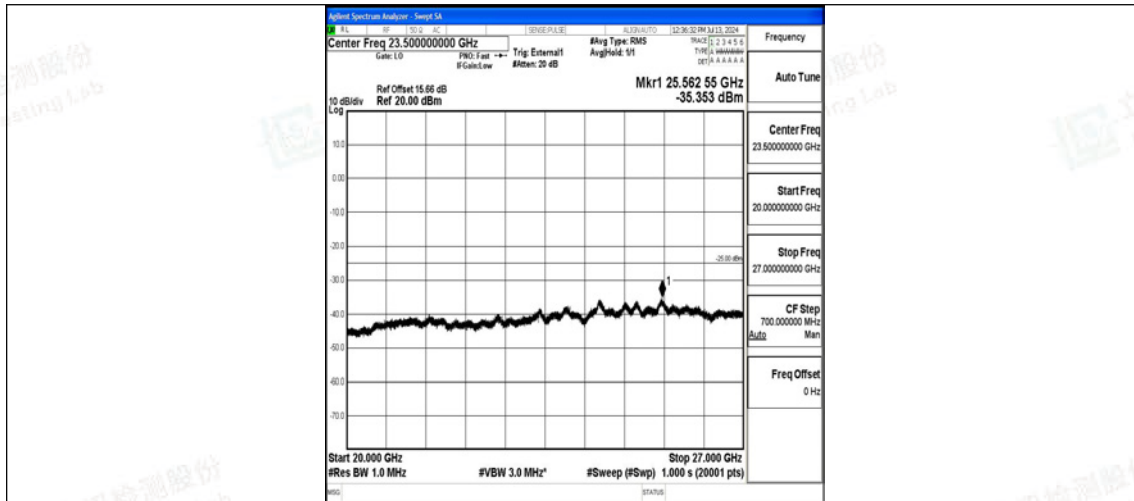
Band41_15MHz_16QAM_39725_1RB#0_20000~27000_20000~27000
