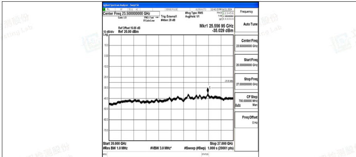
Band41_15MHz_QPSK_41515_1RB#0_20000~27000_20000~27000
