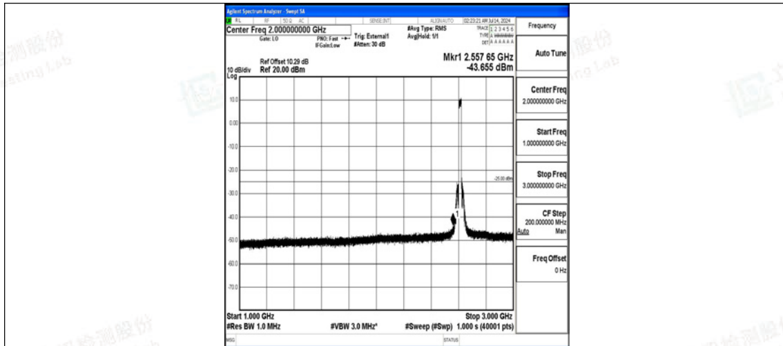
Band38-20MHz-16QAM-38150-100RB#0-1000~3000-PASS
