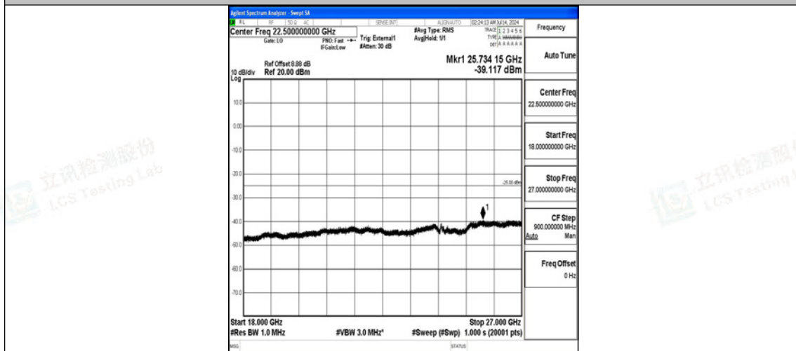
Band38-20MHz-16QAM-38150-100RB#0-18000~27000-PASS
