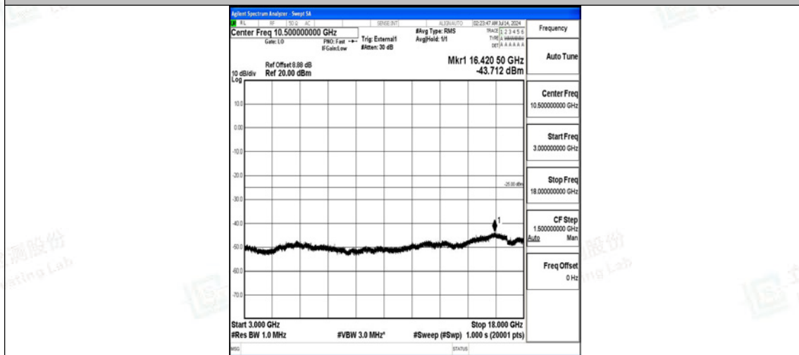
Band38-20MHz-16QAM-38150-100RB#0-3000~18000-PASS
