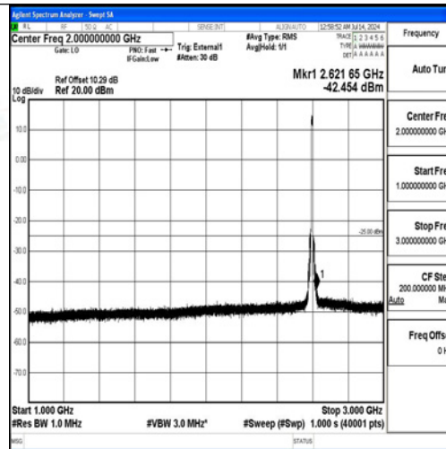
Band38-10MHz-QPSK-38000-50RB#0-1000~3000-PASS
