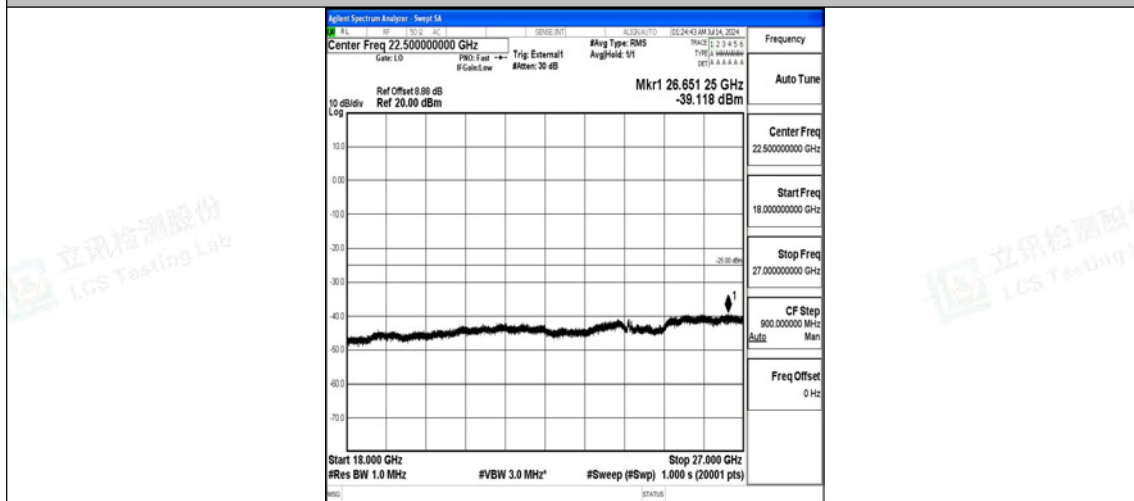
Band38-15MHz-QPSK-37825-75RB#0-18000~27000-PASS
