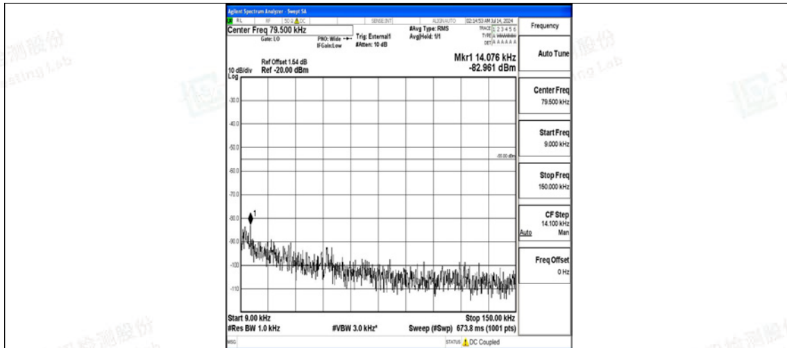
Band38-20MHz-QPSK-38000-100RB#0-0.009~0.15-PASS
