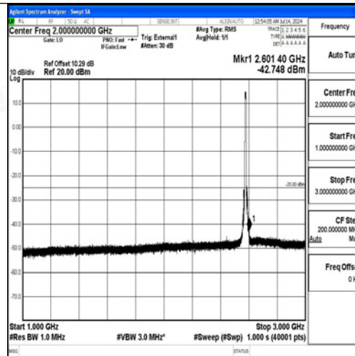
Band38-10MHz-QPSK-37800-50RB#0-1000~3000-PASS
