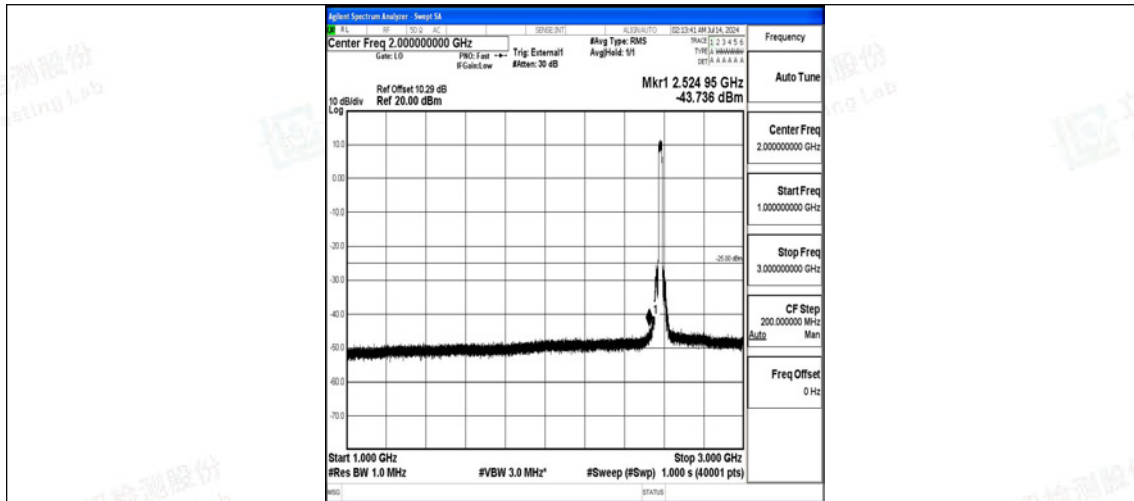
Band38-20MHz-16QAM-37850-100RB#0-1000~3000-PASS
