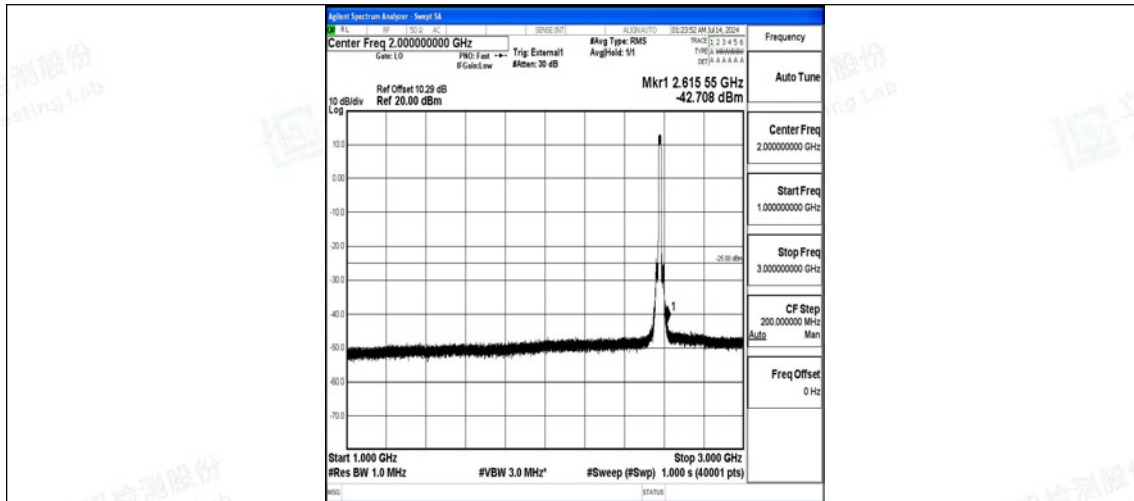
Band38-15MHz-QPSK-37825-75RB#0-1000~3000-PASS
