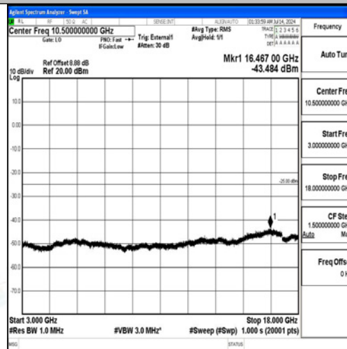
Band38-15MHz-QPSK-38175-75RB#0-3000~18000-PASS
