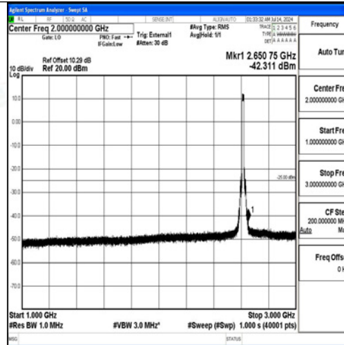
Band38-15MHz-QPSK-38175-75RB#0-1000~3000-PASS
