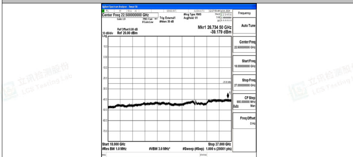
Band38-5MHz-QPSK-37775-25RB#0-18000~27000-PASS
