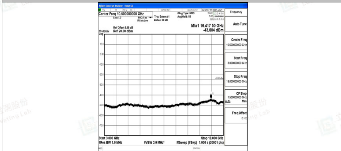
Band38-20MHz-16QAM-37850-100RB#0-3000~18000-PASS
