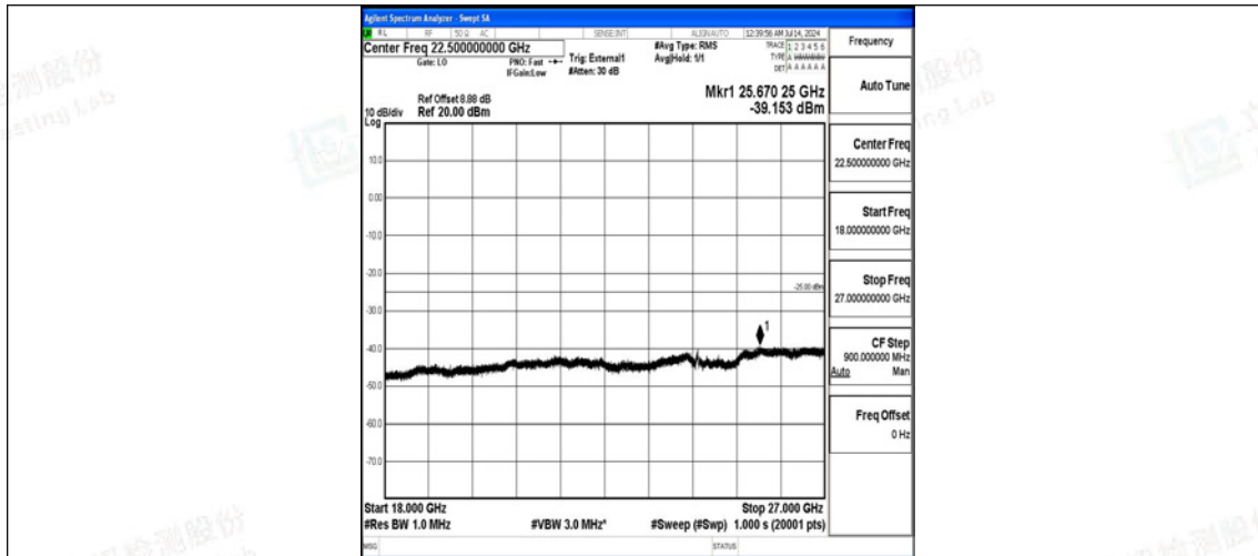
Band38-5MHz-16QAM-38225-25RB#0-18000~27000-PASS
