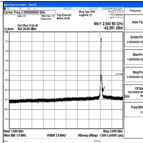
Band38-10MHz-QPSK-38200-50RB#0-1000~3000-PASS
