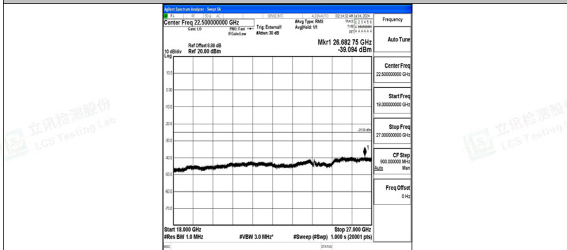
Band38-20MHz-16QAM-37850-100RB#0-18000~27000-PASS
