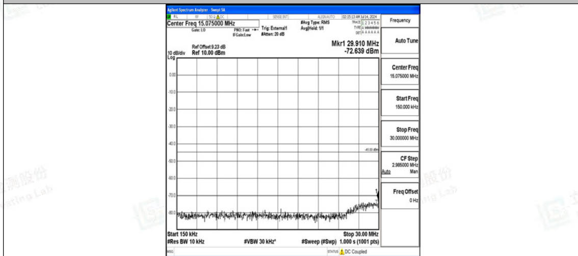
Band38-20MHz-QPSK-38000-100RB#0-0.15~30-PASS
