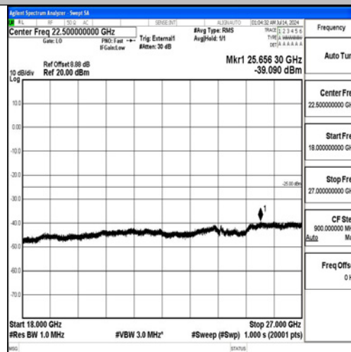
Band38-10MHz-QPSK-38200-50RB#0-18000~27000-PASS
