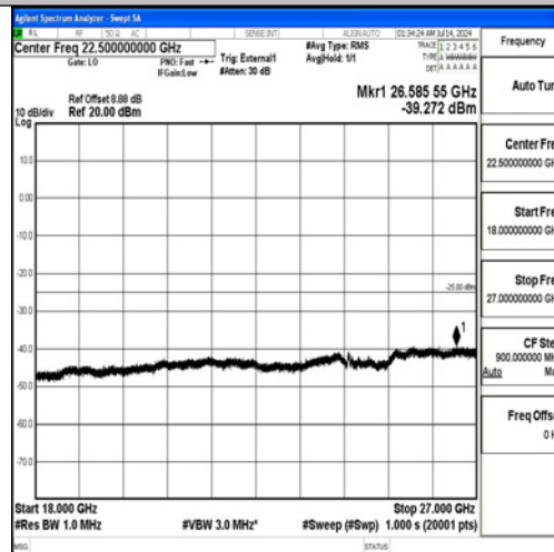
Band38-15MHz-QPSK-38175-75RB#0-18000~27000-PASS
