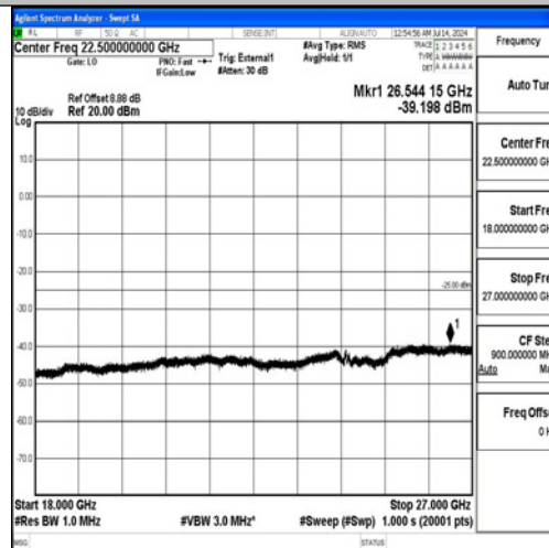
Band38-10MHz-QPSK-37800-50RB#0-18000~27000-PASS
