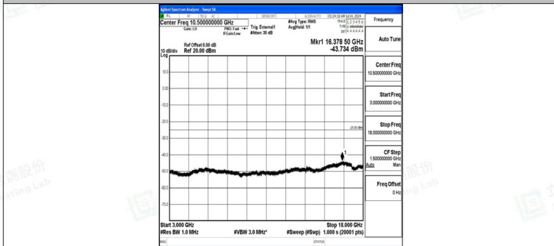
Band38-15MHz-QPSK-37825-75RB#0-3000~18000-PASS
