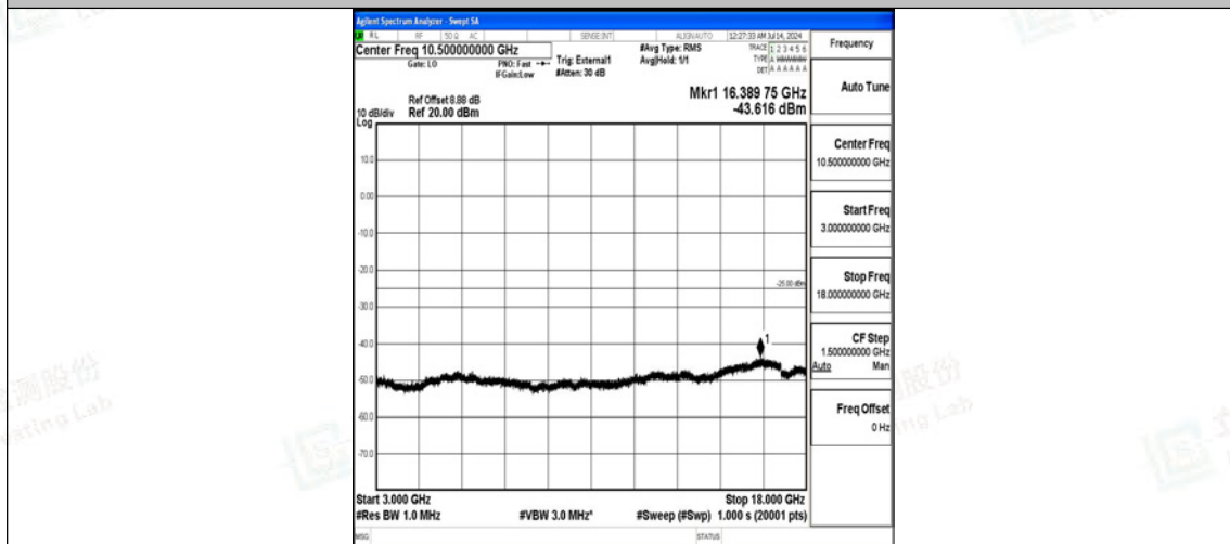
Band38-5MHz-QPSK-37775-25RB#0-3000~18000-PASS
