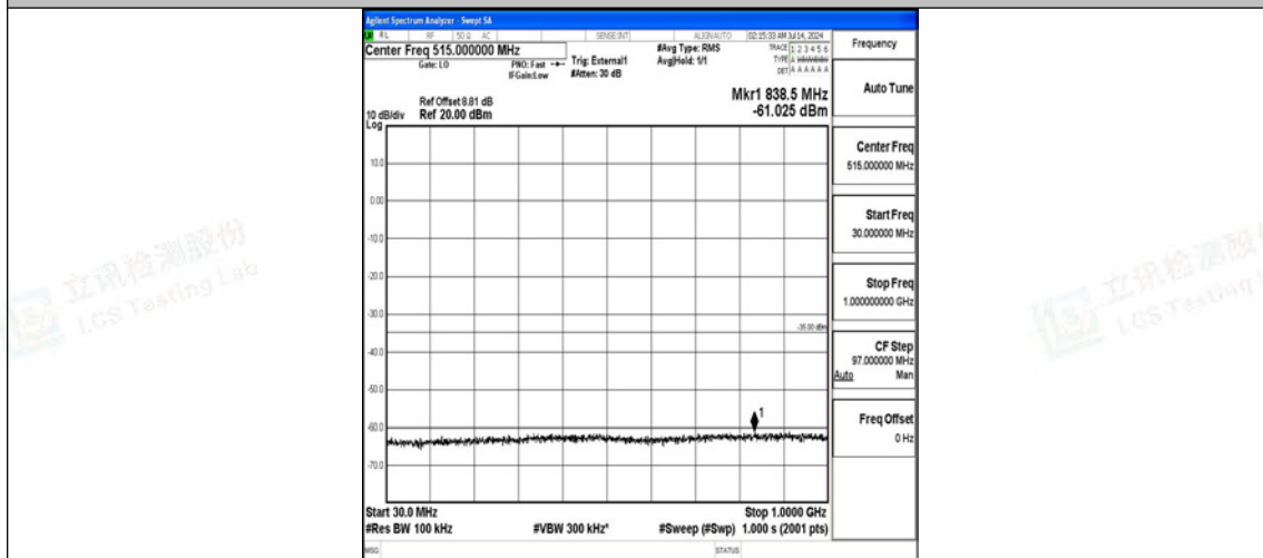
Band38-20MHz-QPSK-38000-100RB#0-30~1000-PASS
