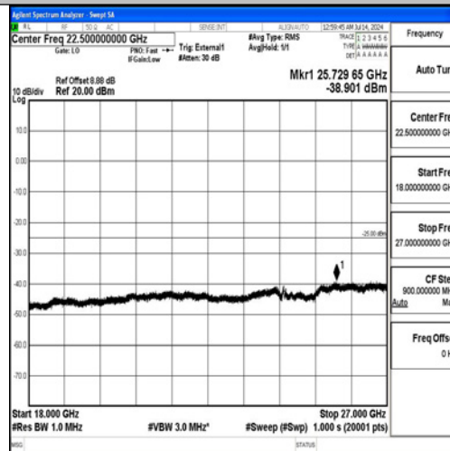
Band38-10MHz-QPSK-38000-50RB#0-18000~27000-PASS
