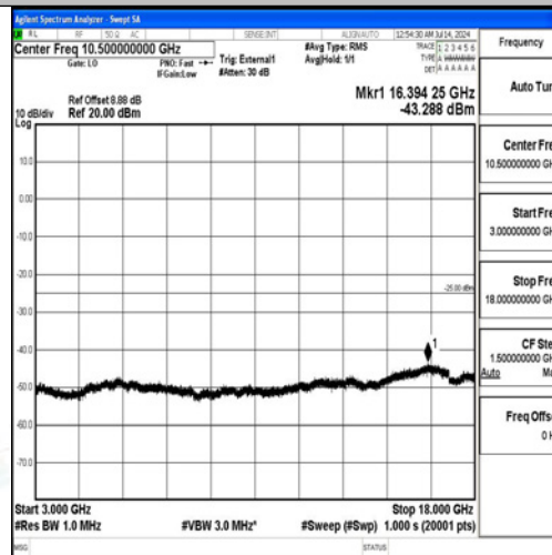
Band38-10MHz-QPSK-37800-50RB#0-3000~18000-PASS
