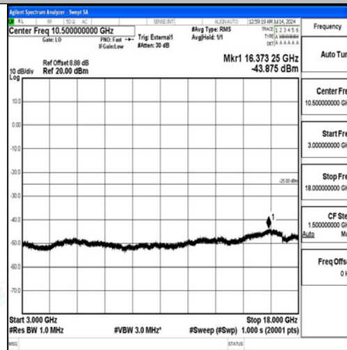
Band38-10MHz-QPSK-38000-50RB#0-3000~18000-PASS
