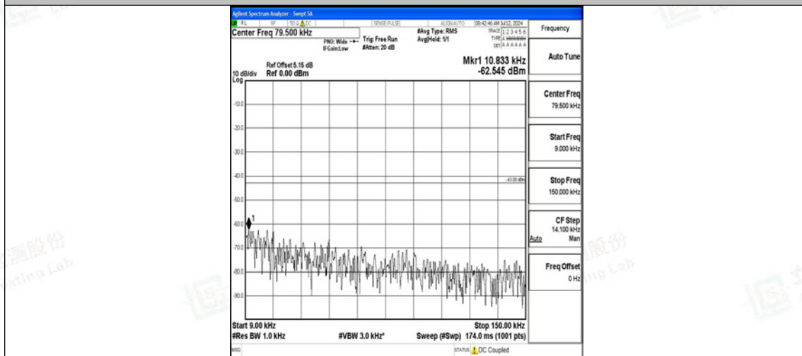
Band25_20MHz_16QAM_26590_1RB#0_0.009~0.15_0.009~0.15
