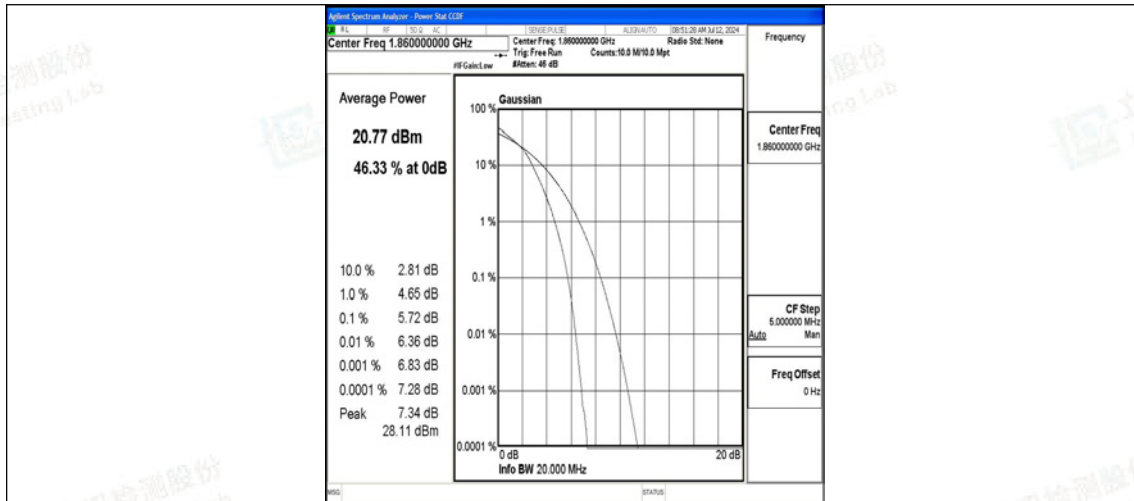
Band25-20MHz-16QAM-26140-100RB#0-PASS
