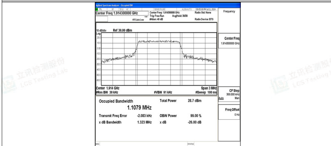
Band25-1.4MHz-16QAM-26683-6RB#0-PASS
