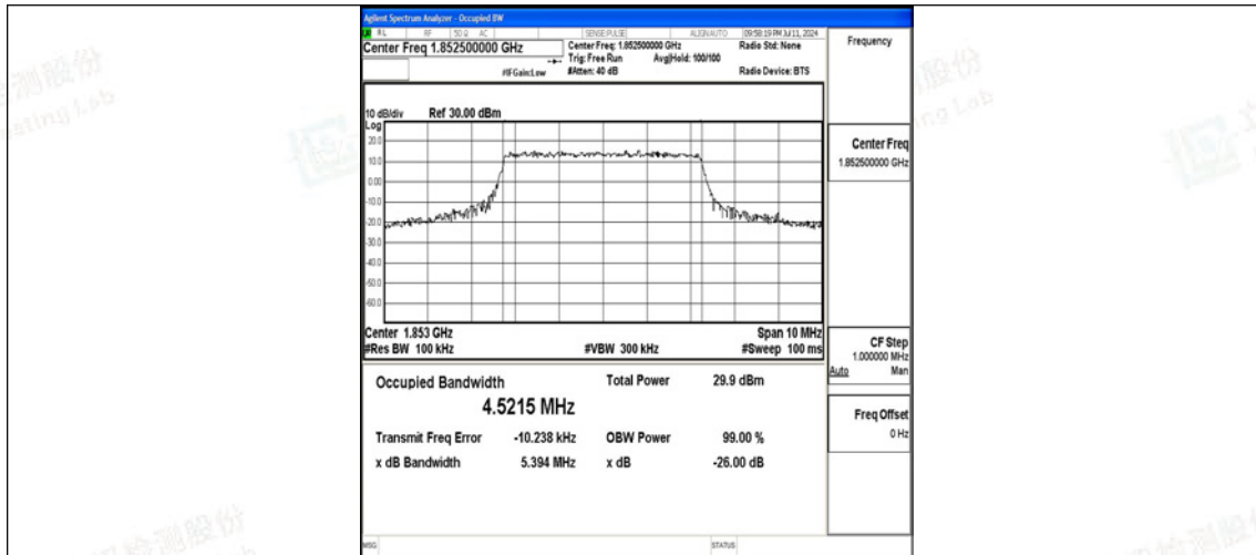
Band25-5MHz-QPSK-26065-25RB#0-PASS
