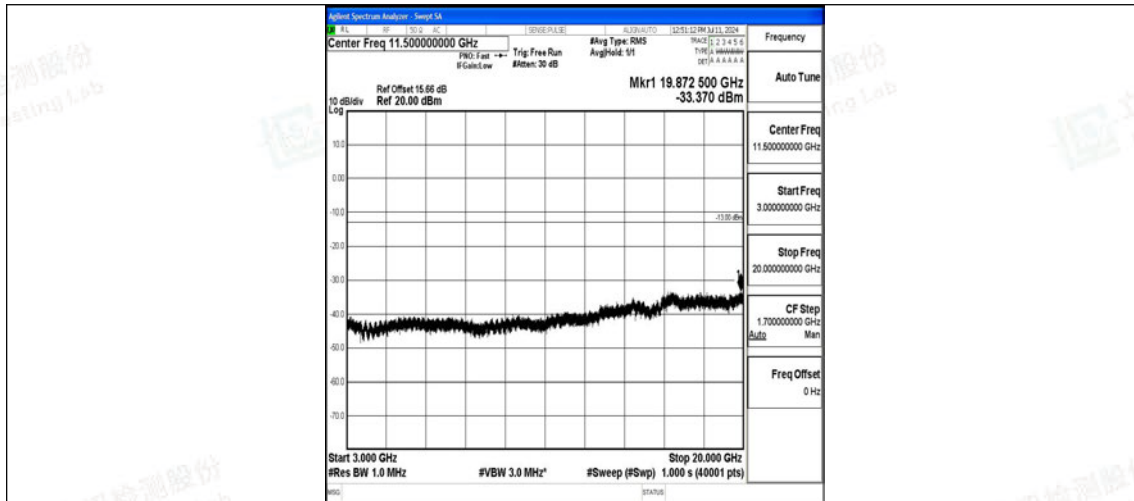
Band2_20MHz_16QAM_18700_1RB#0_3000~20000_3000~20000
