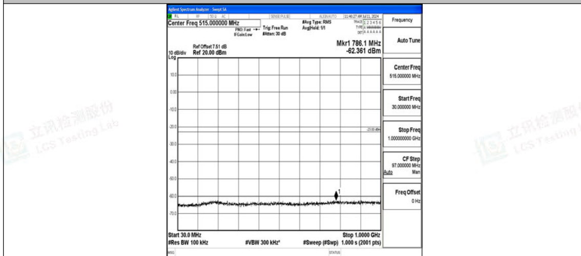
Band2_5MHz_QPSK_18625_1RB#0_30~1000_30~1000
