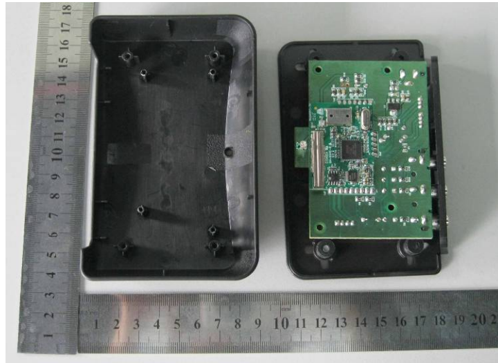
EUT – Uncovered View
