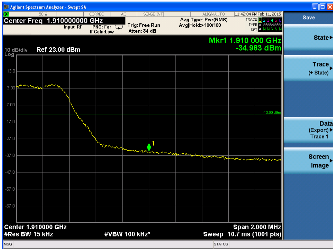
CDMA PCS +F-SCH 1175 Channel
