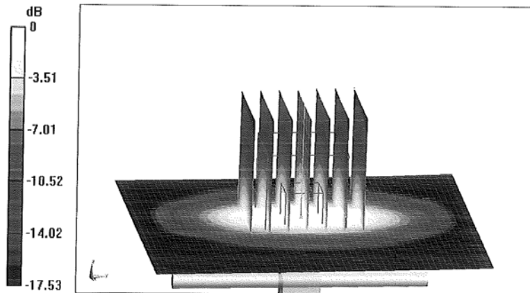
0 dB = 14.4 W/kg = 11.58 dBW/kg
