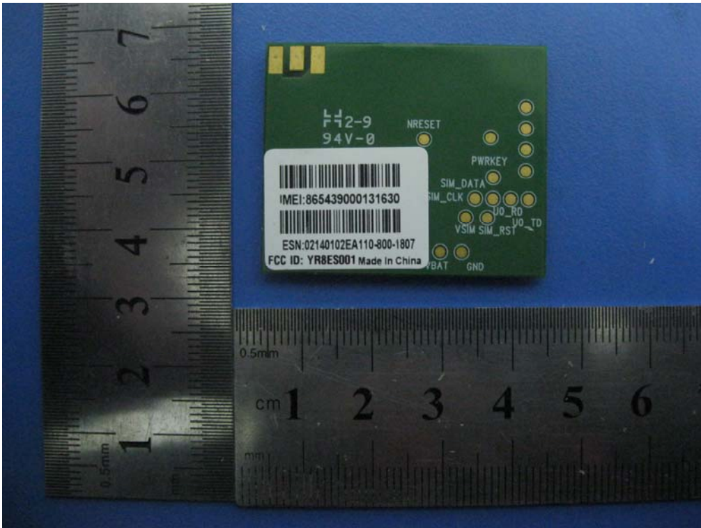
GSM Module PCB Board – Bottom View
