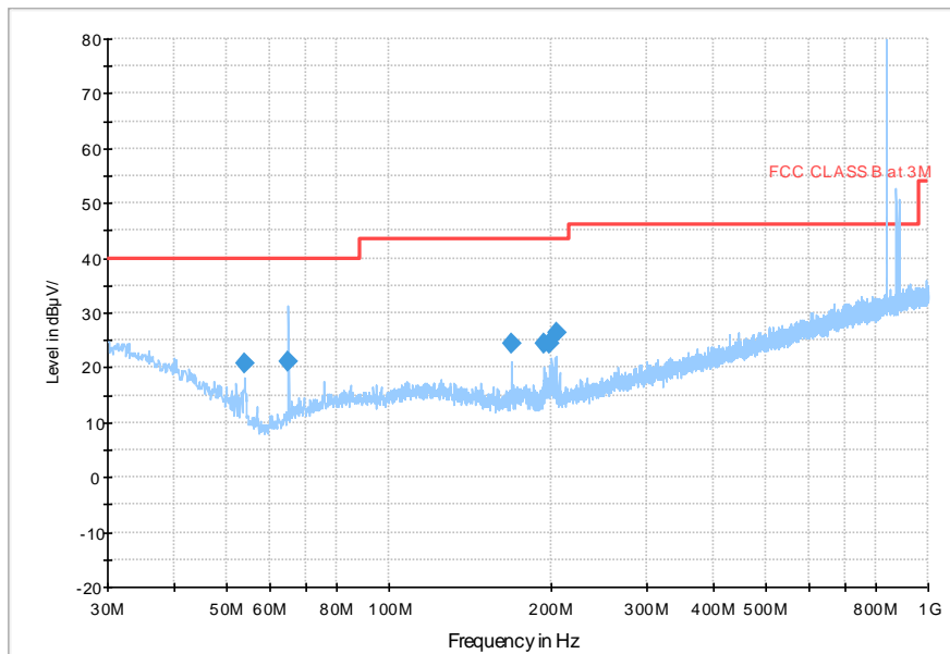
(Plot B: Test Antenna Horizontal Frequency from 30MHz to1GHz)
