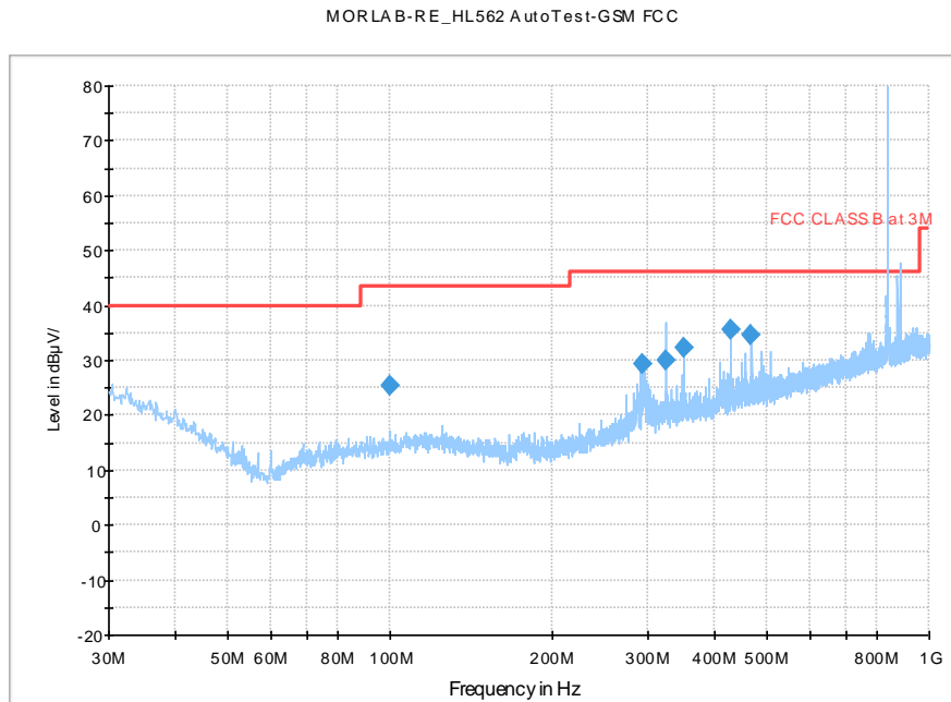
(Plot A: Test Antenna Vertical Frequence from 30MHz to1GHz)
