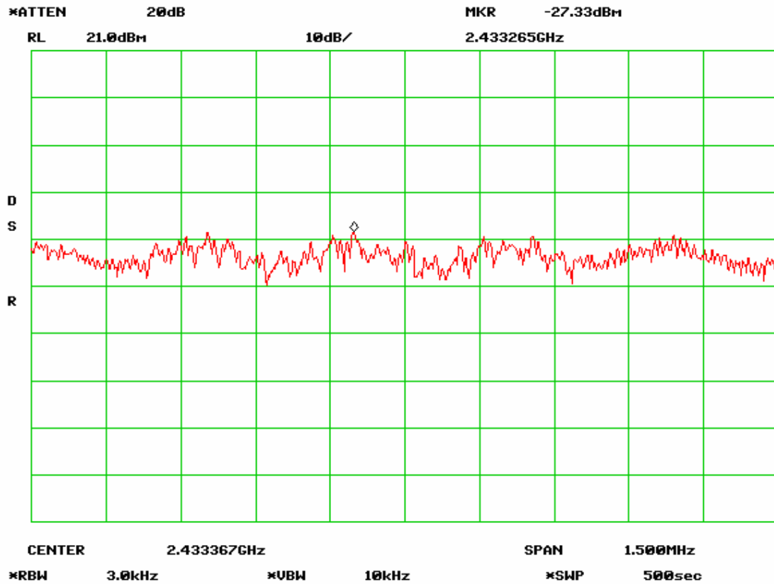
PSD - Middle Channel (802.11n-20MHz) chain 2
