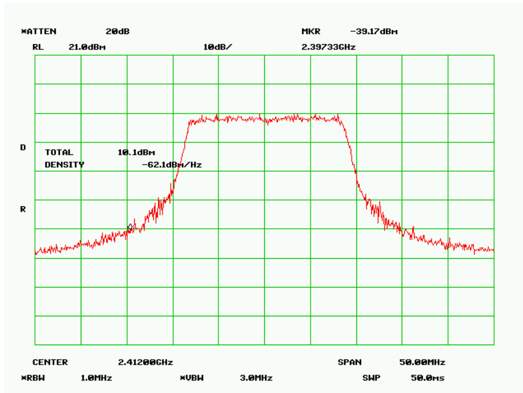
Output Power Low Channel (802.11n-20MHz) chain 2
