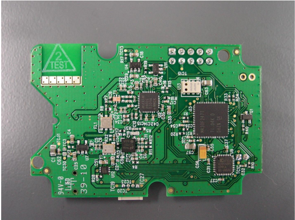
Circuit board bottom w/o shield
