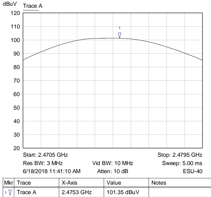
Graph 6: Highest Channel Output Power Plot
