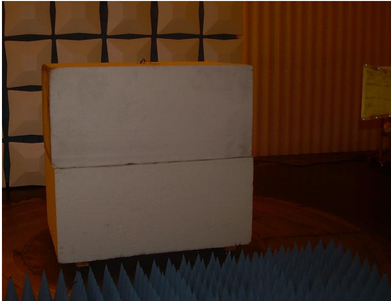
Photograph 5: Front View Radiated Emissions – Above 1000 MHz
