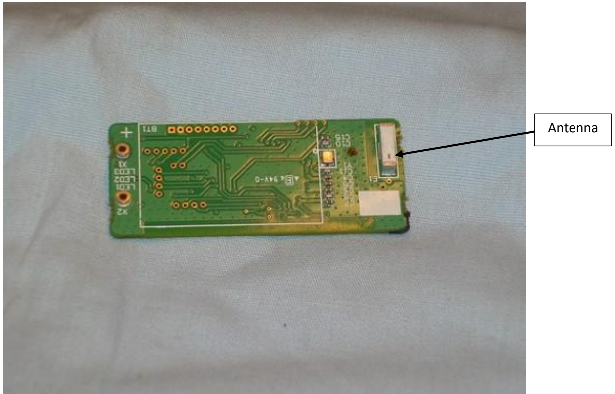
Photograph 2 – Back View of the Device with Battery Removed
