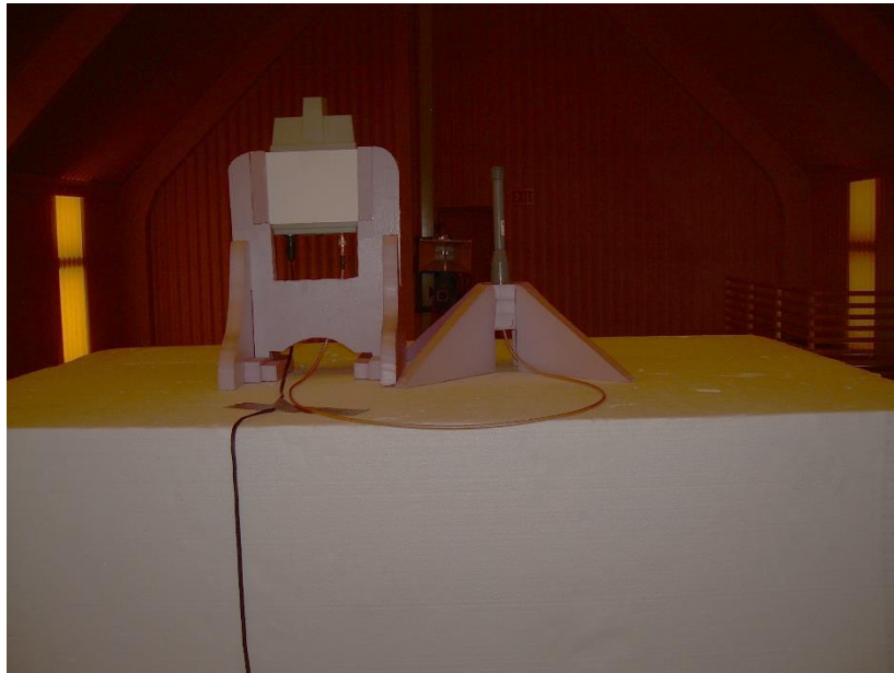
Photograph 4: Back View Radiated Emissions – Above 1000 MHz – HGV-2404U Antenna
