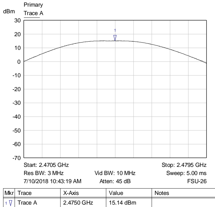
Graph 6: Highest Channel Output Power Plot
