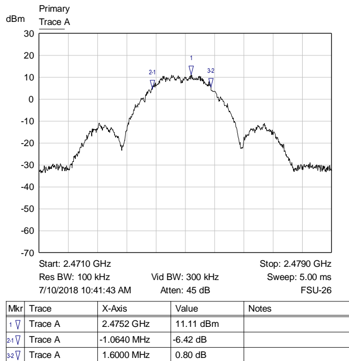
Graph 3: Highest Channel Bandwidth
