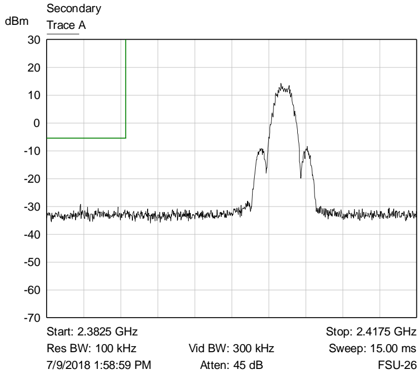
Graph 26: Lower Band Edge Plot
