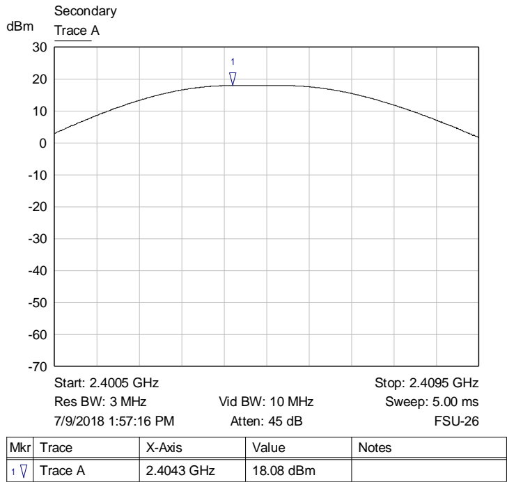
Graph 23: Lowest Channel Output Power Plot
