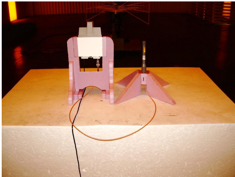
Photograph 2: Back View Radiated Emissions Worst-Case Configuration – 30 MHz – 1000 MHz
