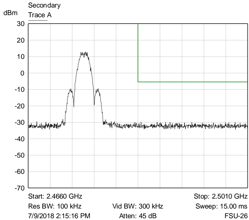
Graph 27: Upper Band Edge Plot
