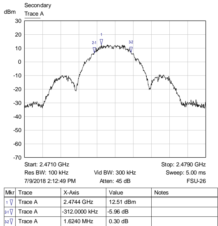
Graph 22: Highest Channel Bandwidth
