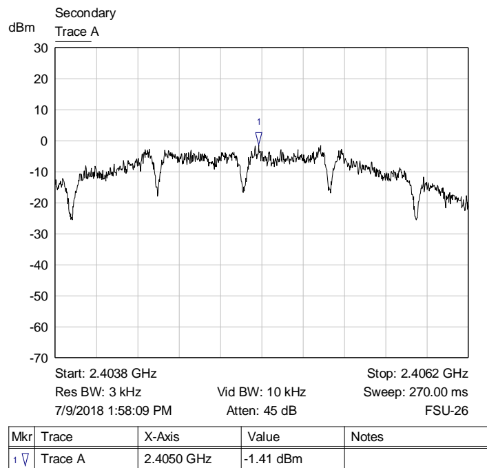
Graph 30: Lowest Channel 3 kHz PSD Plot
