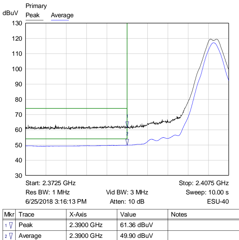
Graph 11: Radiated Lower Band Edge Plot – HG2415U-PRO
