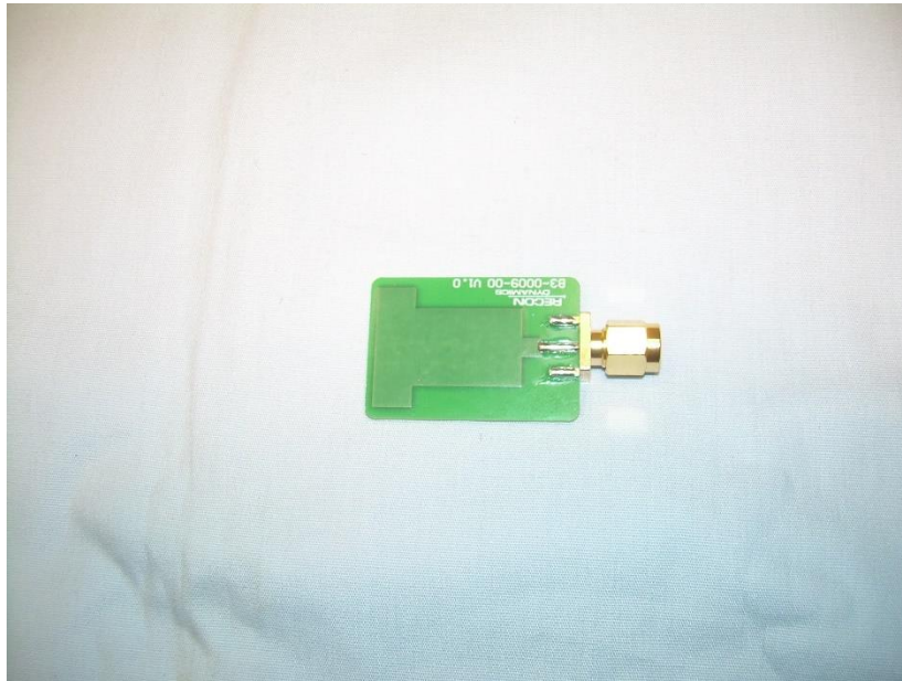
Photograph 26 – View of the Secondary 802.15.4 Transceiver Antenna – Front
