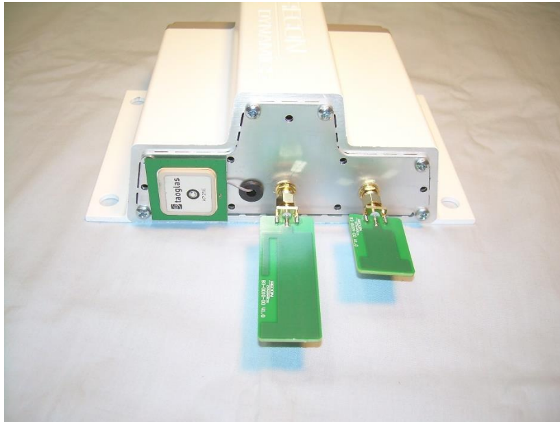
Photograph 16 – View of the GPS Antenna, Cell Module Antenna, and Secondary 802.15.4 Transceiver Antenna that Mount Under Top Cover
