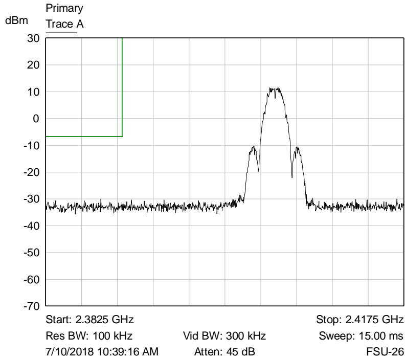
Graph 7: Lower Band Edge Plot
