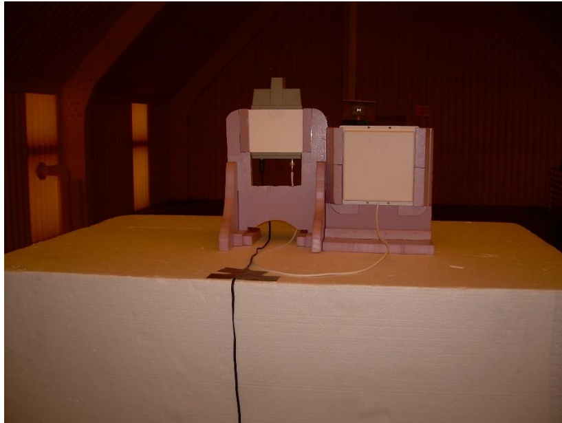
Photograph 5: Radiated Emissions – RE14U Antenna
