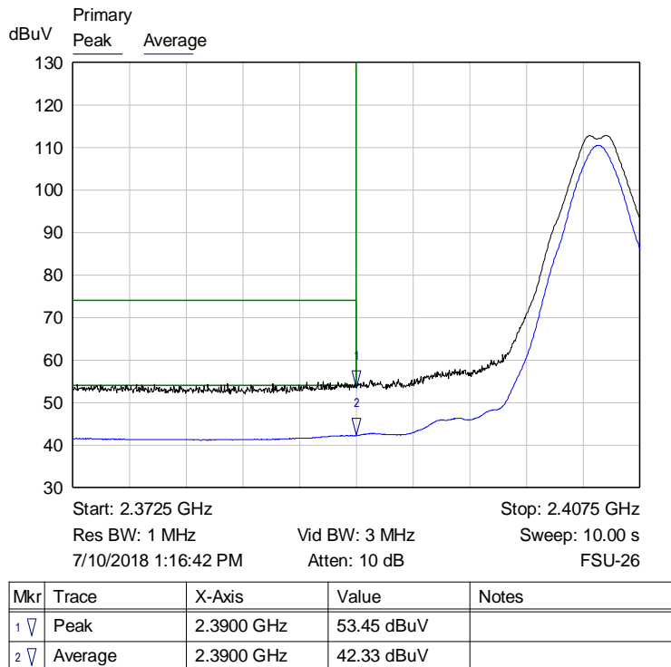
Graph 15: Radiated Lower Band Edge Plot – HGV-2404U Antenna
