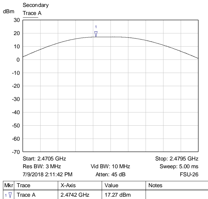
Graph 25: Highest Channel Output Power Plot
