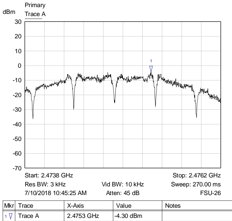
Graph 19: Highest Channel Output 3 kHz PSD Plot
