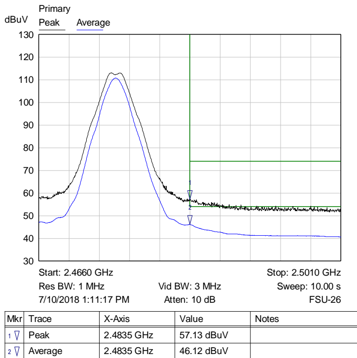
Graph 16: Radiated Upper Band Edge Plot – HGV-2404U Antenna
