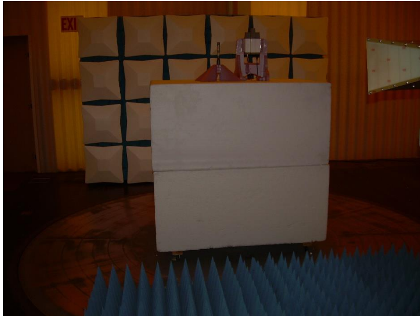
Photograph 3: Front View Radiated Emissions – Above 1000 MHz – HGV-2404U Antenna
