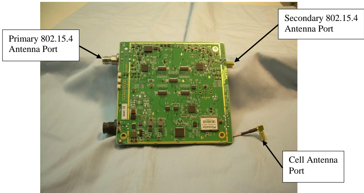
Photograph 19 – View of the Component Side of the PCB
