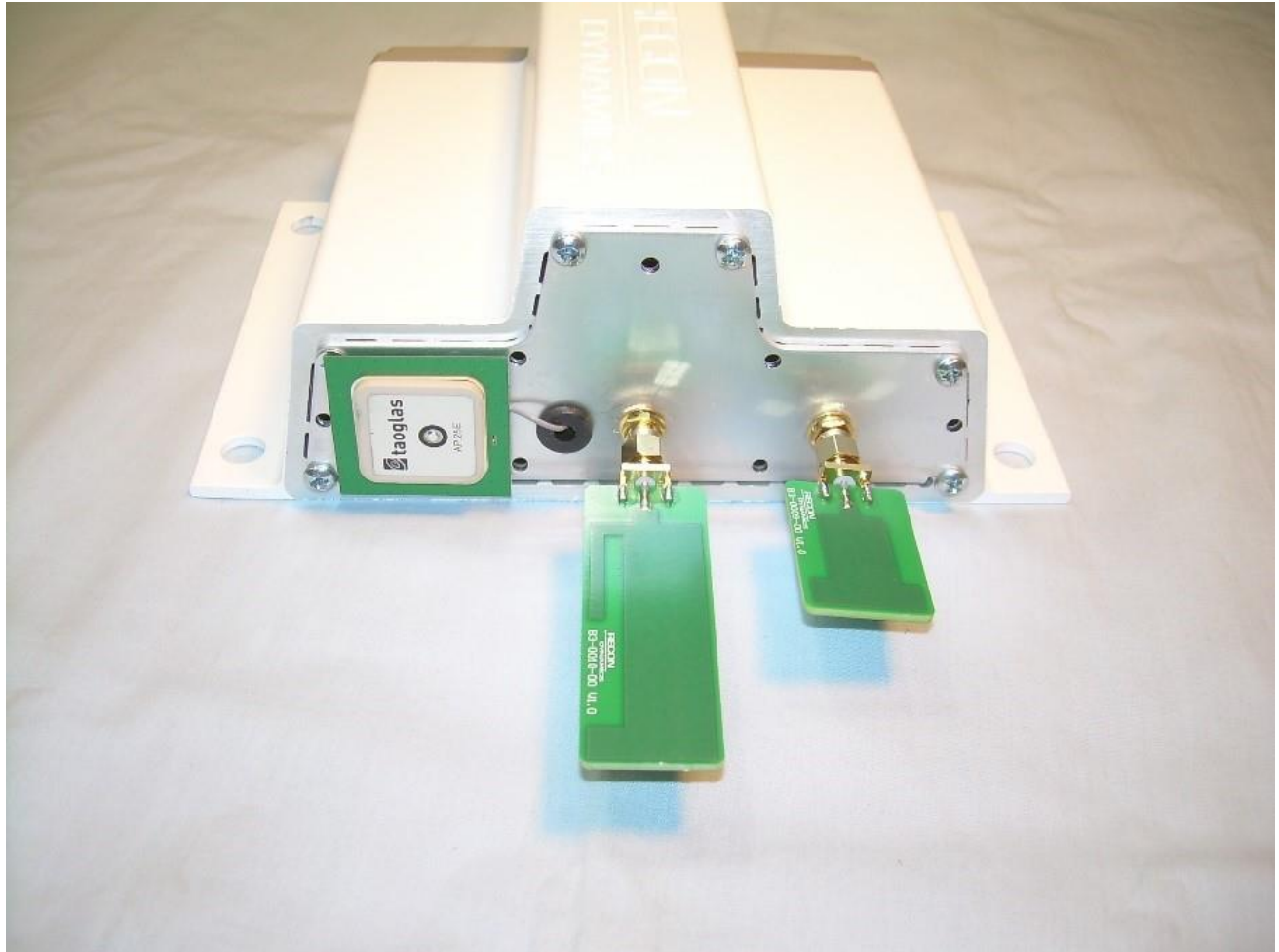
Photograph 7 – View of the GPS Antenna, Cell Module Antenna, and Secondary 802.15.4 Transceiver Antenna that Mount Under Top Cover
