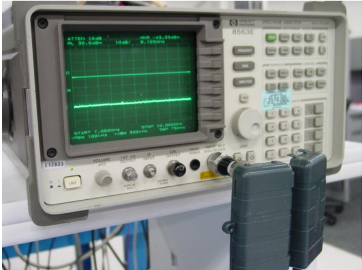
RF Conducted measurement (7000 - 10000 MHz spurious emissions)
