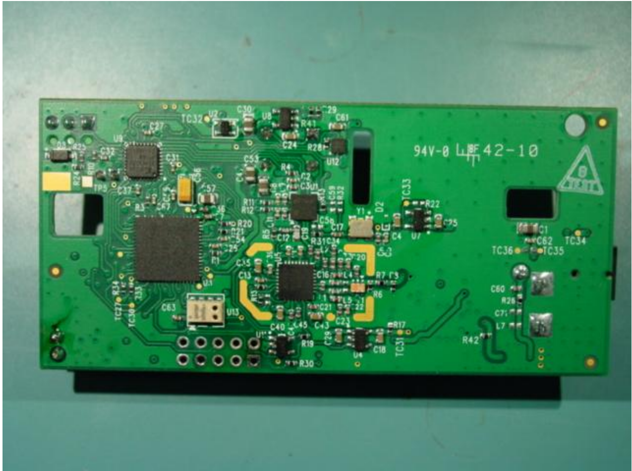
Circuit board bottom without shield
