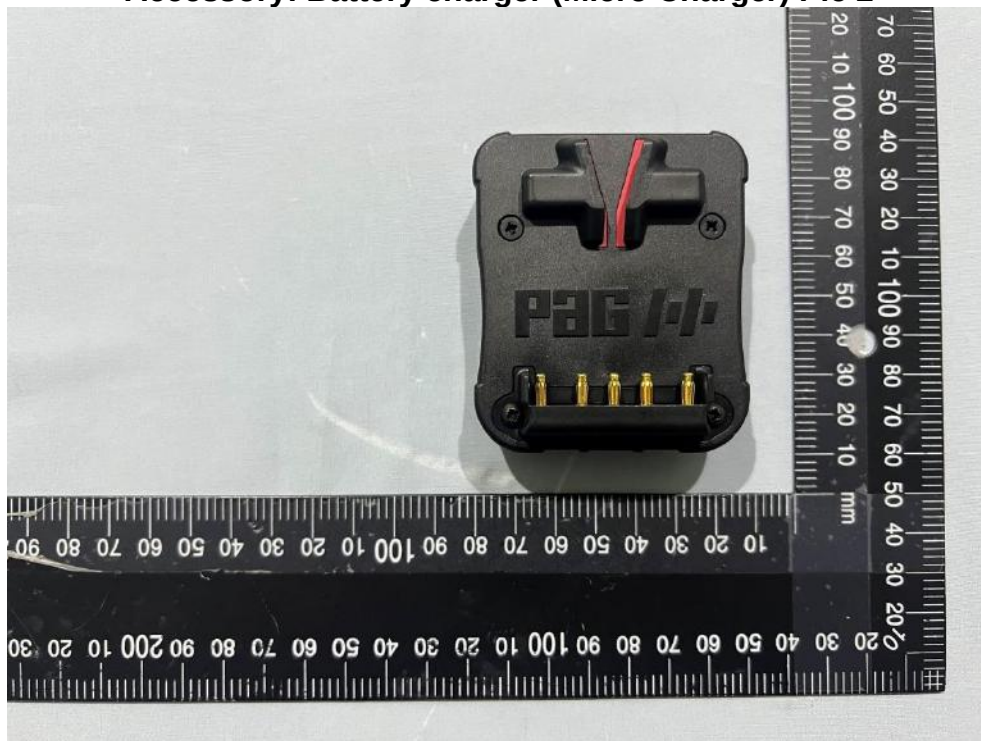
Accessory: Battery charger (Micro Charger) Pic 2
