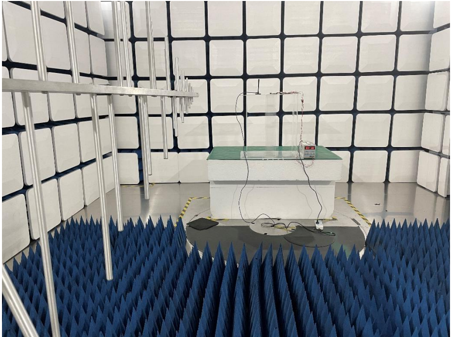
30 MHz-1 GHz
