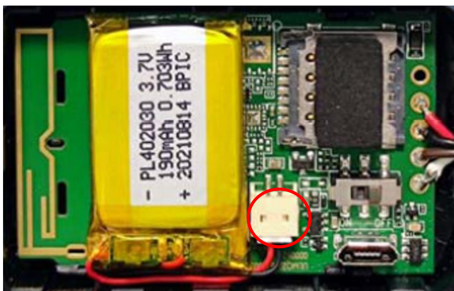
Figure 9. Installing the Internal Backup Battery
