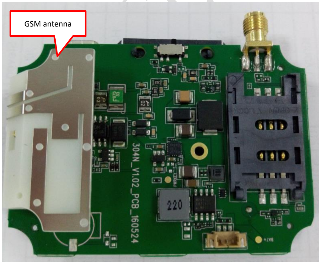
GV304N_Bottom View
