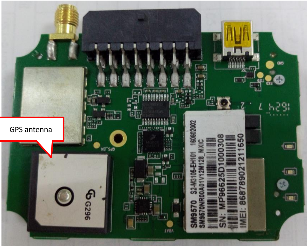
GV304N_Top View
