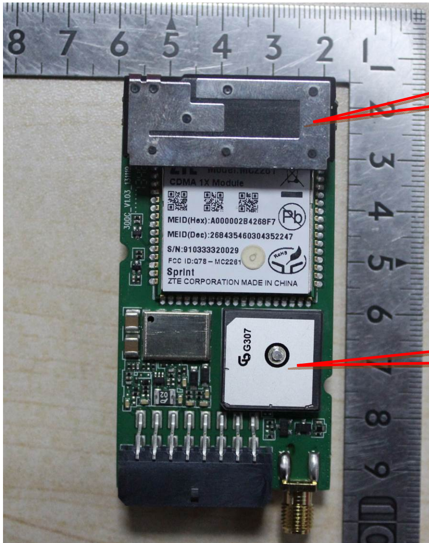
View of EUT-10
