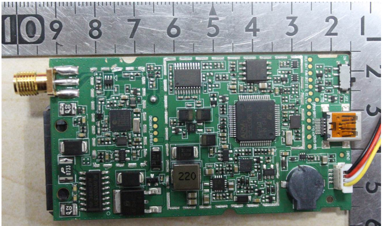
View of EUT-6
