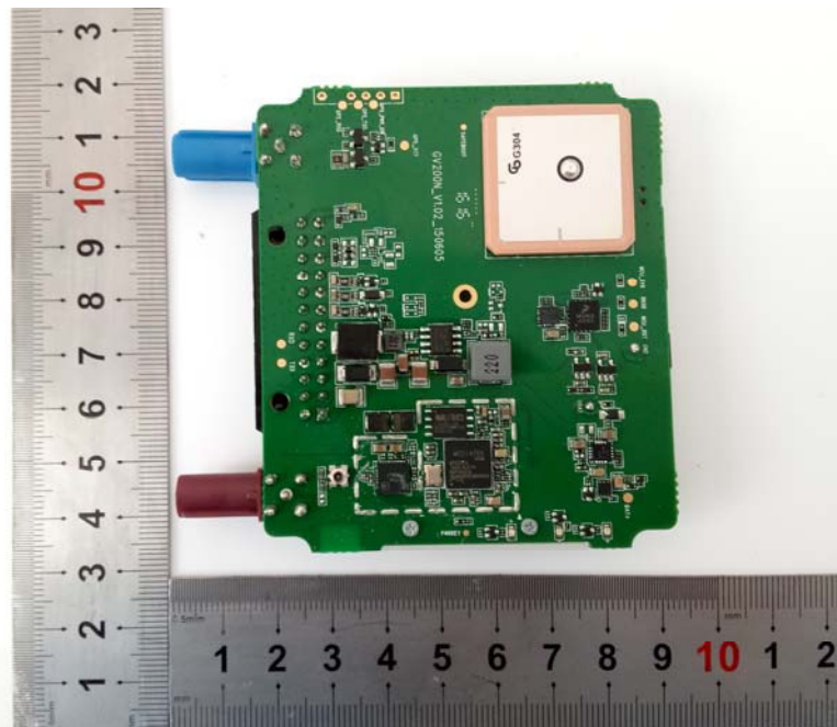
EUT – Main Board Top Shielding off View
