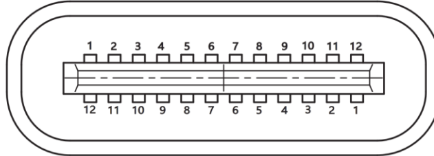
Figure 3. 12-pin (two sides) Type-C Interface of GL502MG
