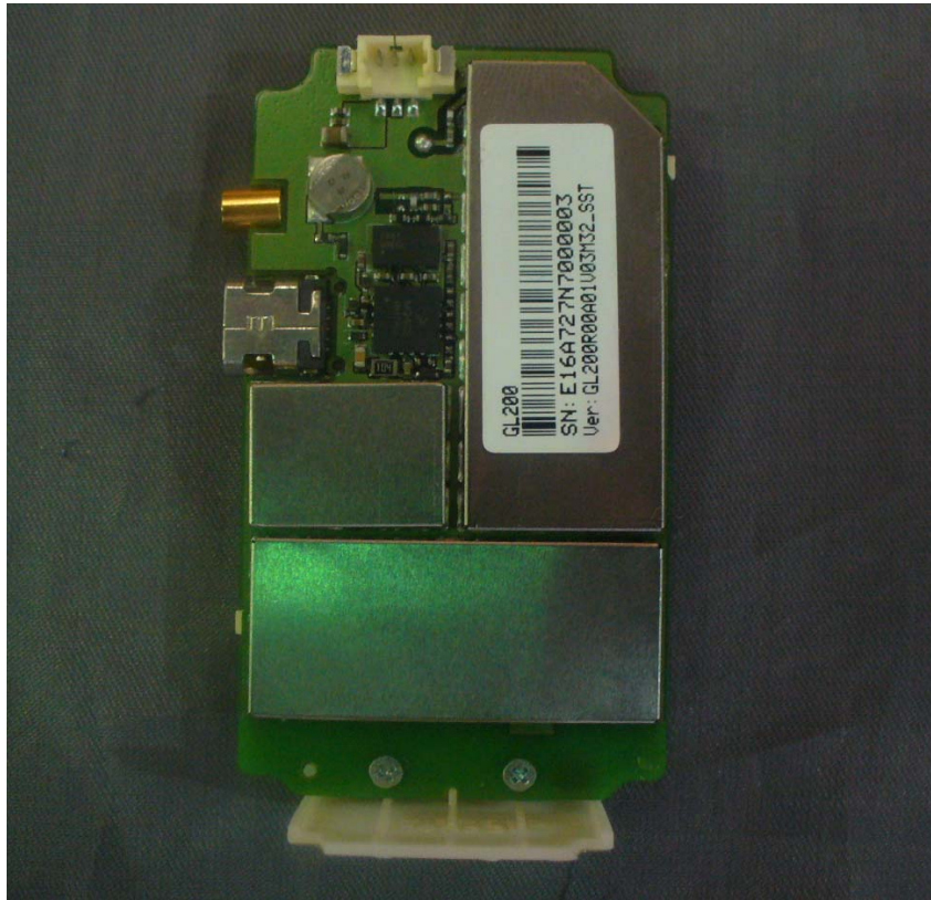
Bottom View
