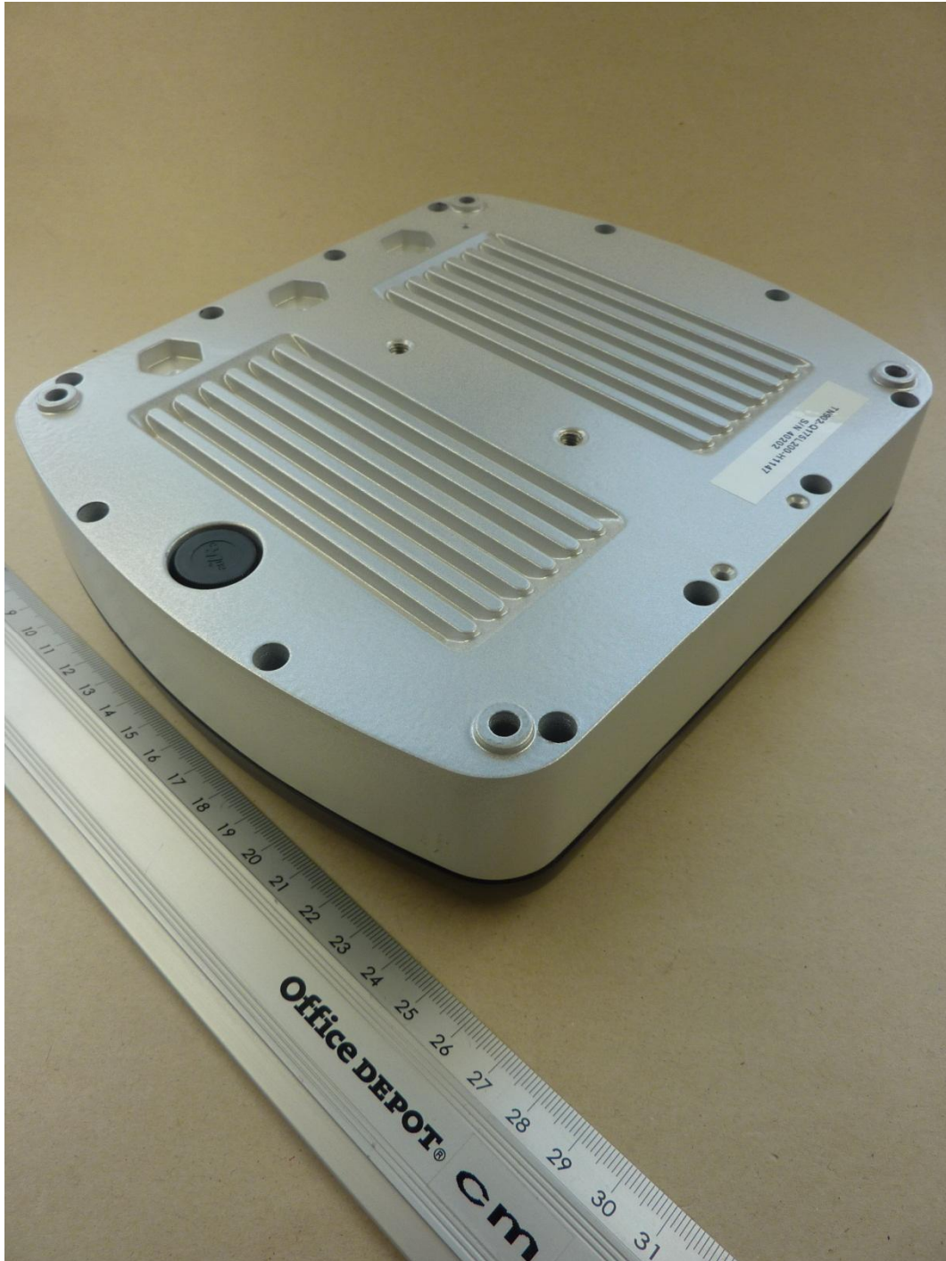
153143_2.JPG: TN902-Q175L200-H1147, 3-D-view 2
