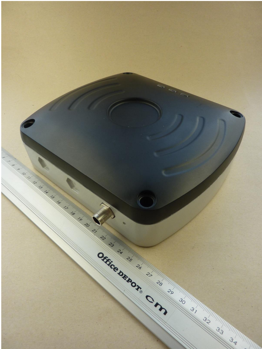
153143_1.JPG: TN902-Q175L200-H1147, 3-D-view 1
