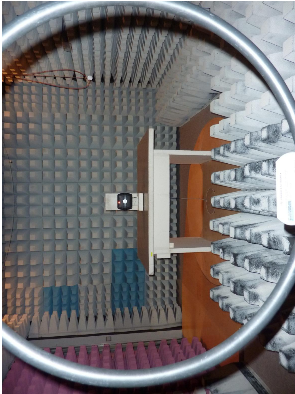
122887_15.JPG: TN902-Q175L200-H1147, test set-up fully anechoic chamber
