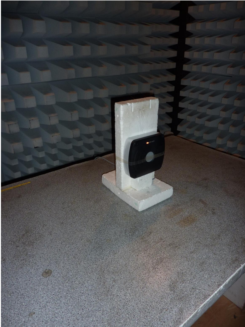
122887_16.JPG: TN902-Q175L200-H1147, test set-up fully anechoic chamber
