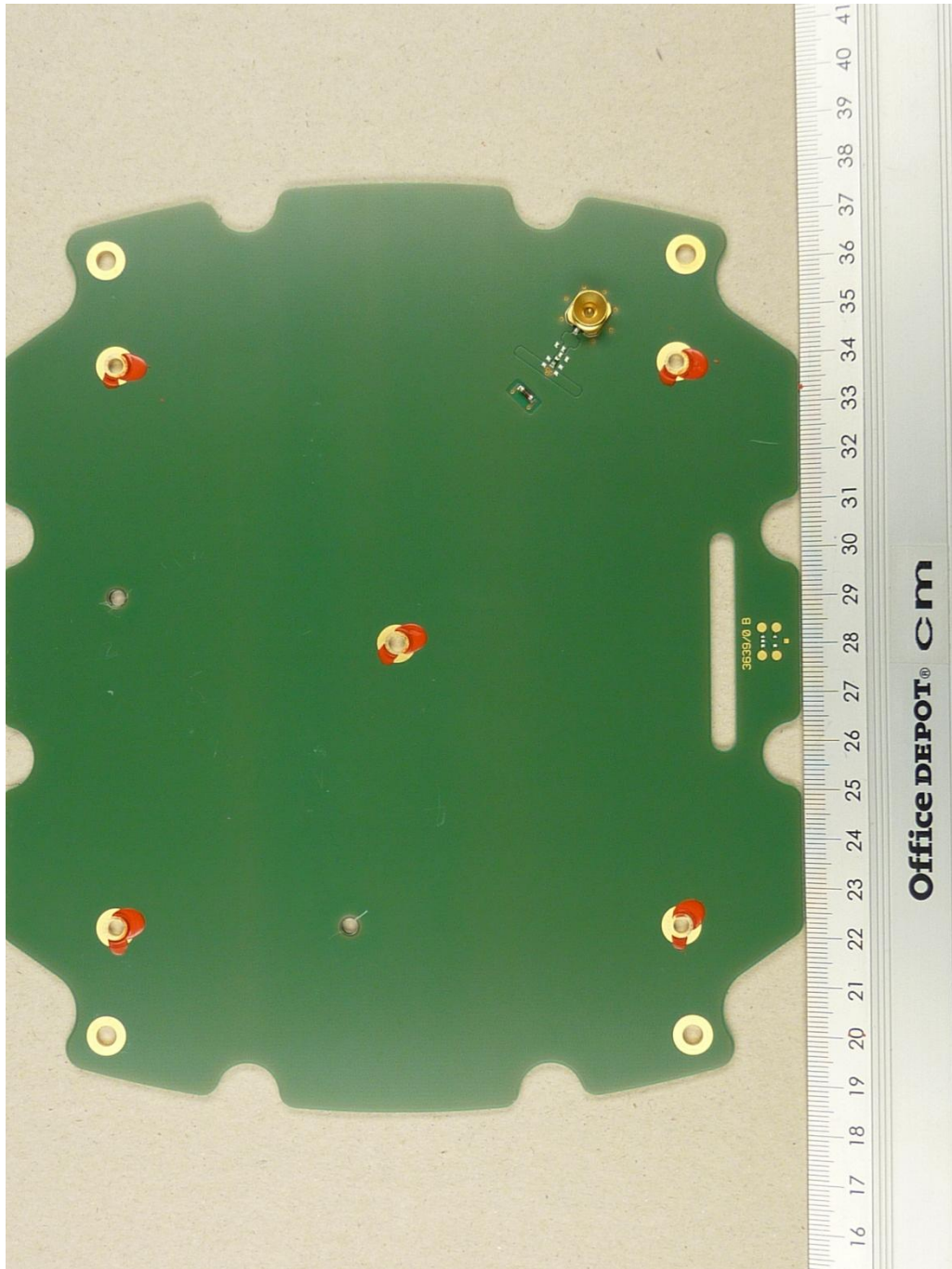
122887_s.JPG: TN902-Q175L200-H1147, coupler PCB, top view
