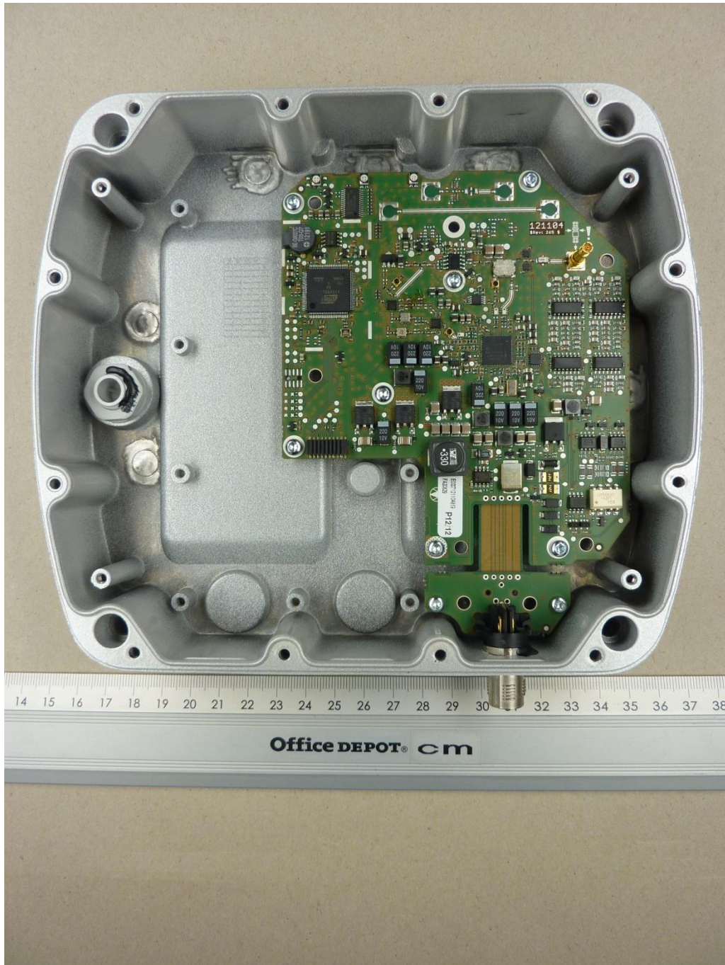
122887_p.JPG: TN902-Q175L200-H1147, internal view 2 (antenna removed)
