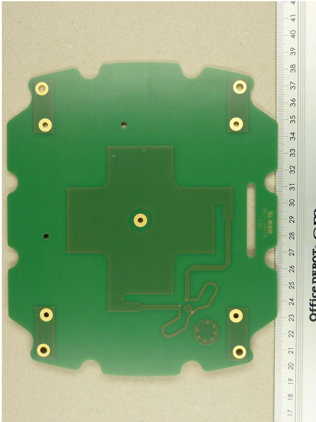
122887_t.JPG: TN902-Q175L200-H1147, coupler PCB, bottom view
