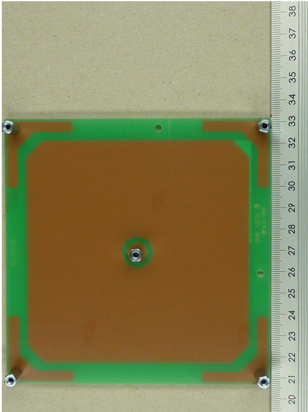
122887_u.JPG: TN902-Q175L200-H1147, antenna PCB, top view
