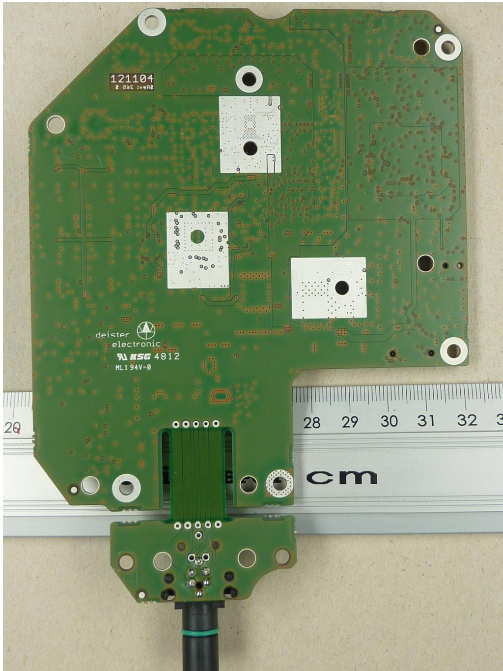
122887_r.JPG: TN902-Q175L200-H1147, main PCB, bottom view
