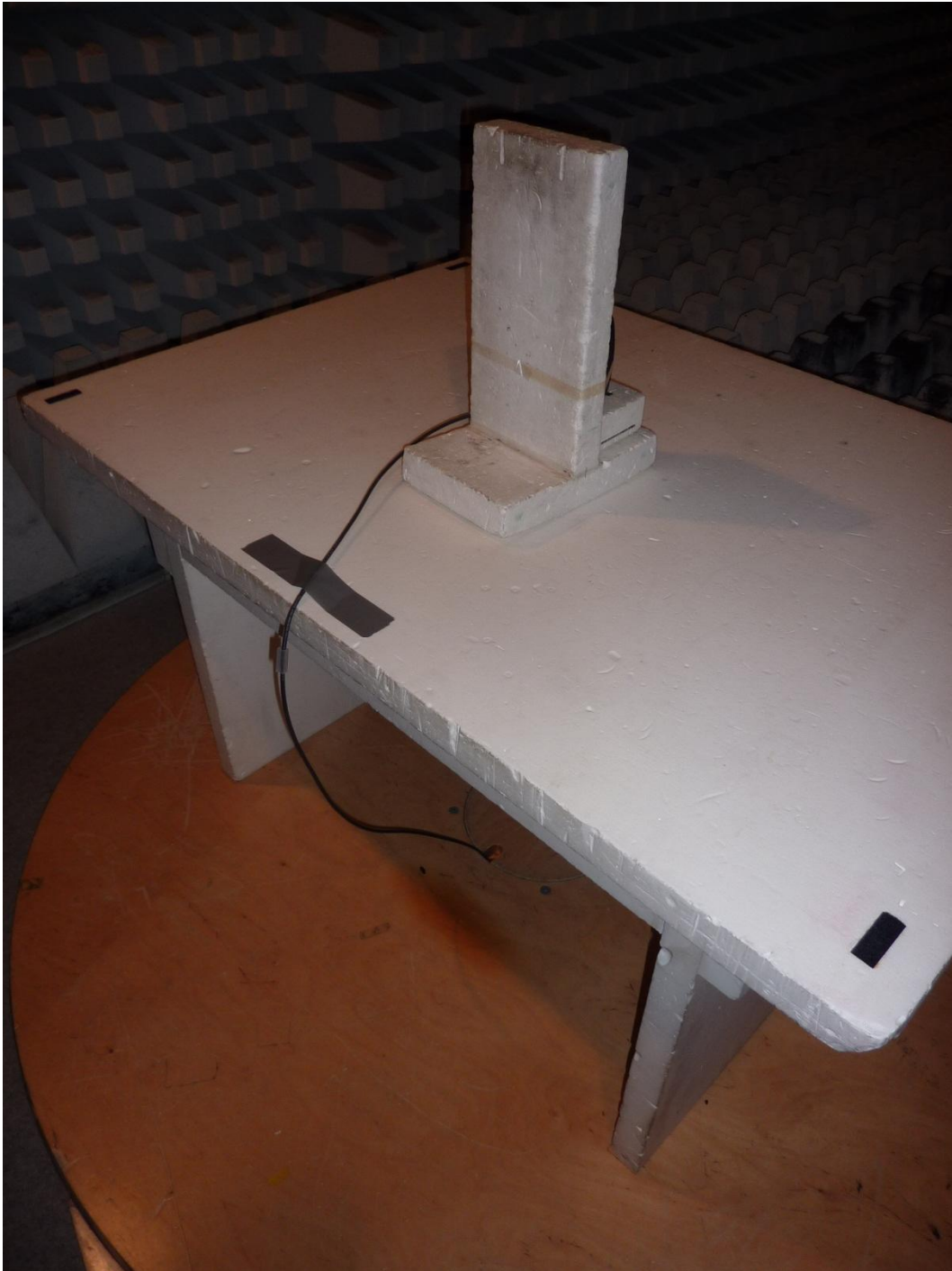
153142_a.JPG: TN902-Q120L130H1147, test setup fully anechoic chamber
