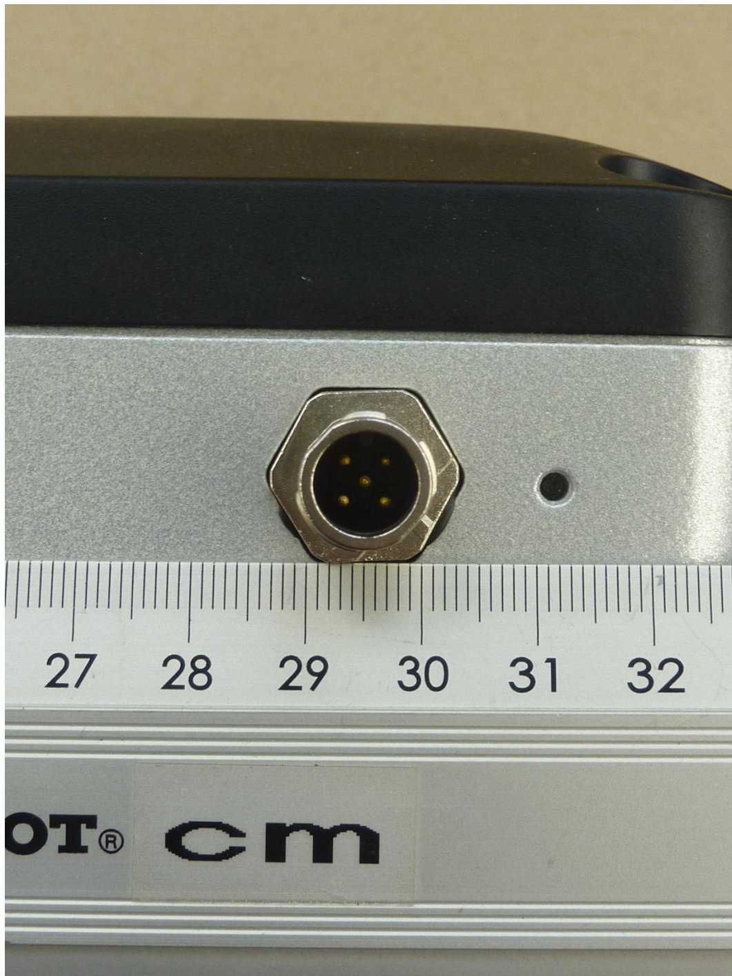
153142_4.JPG: TN902-Q120L130H1147, connector view
