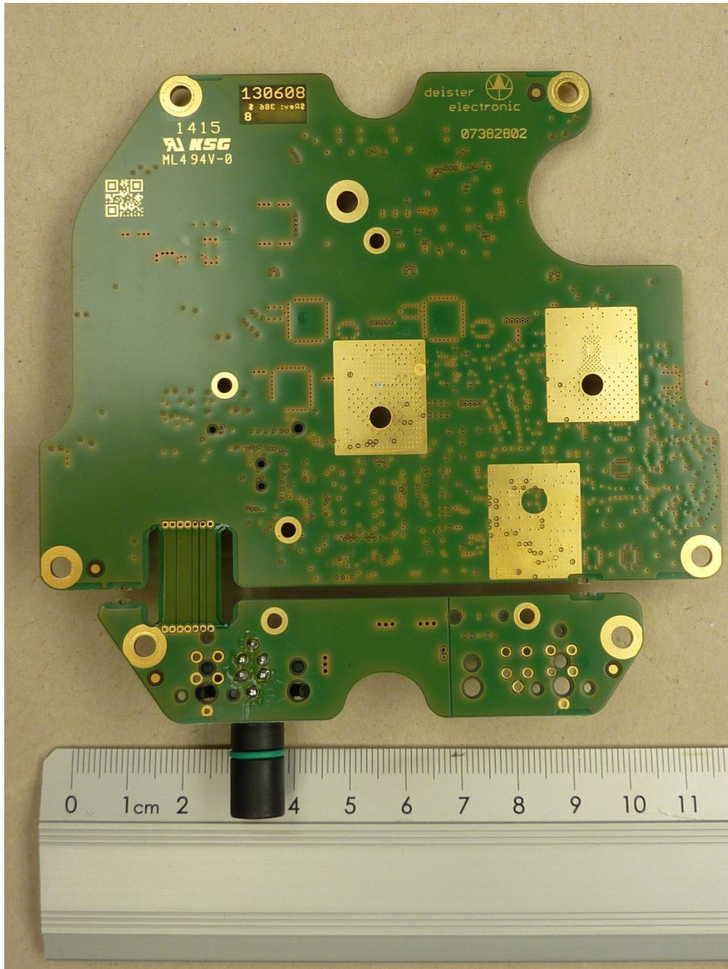
142568_11.JPG: TN902-Q120L130-H1147, main PCB, bottom view
