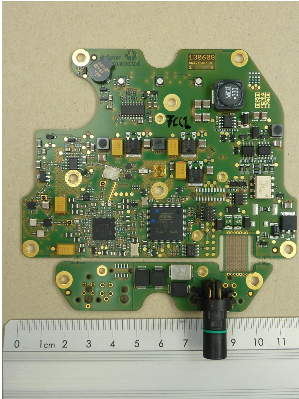
142568_10.JPG: TN902-Q120L130-H1147, main PCB, top view
