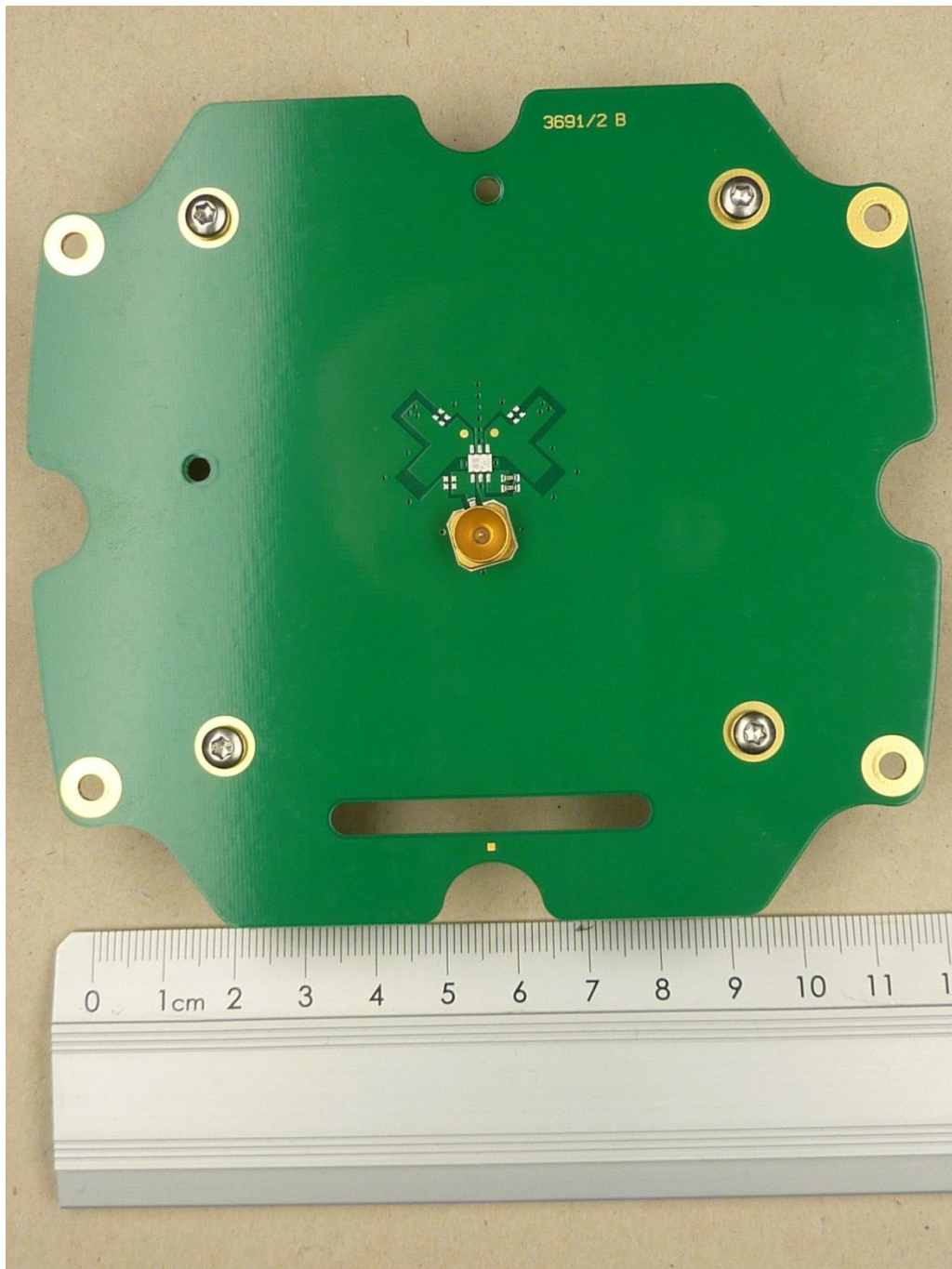
142568_5.JPG: TN902-Q120L130-H1147, coupler PCB, bottom view
