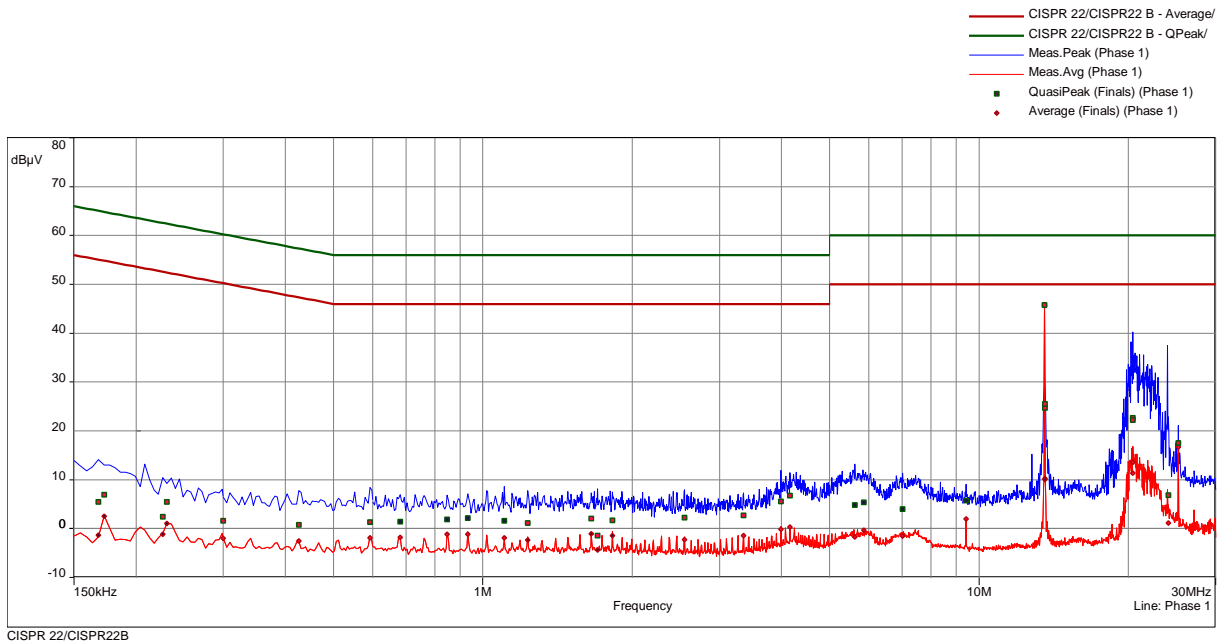
CISPR 22/CISPR22B
